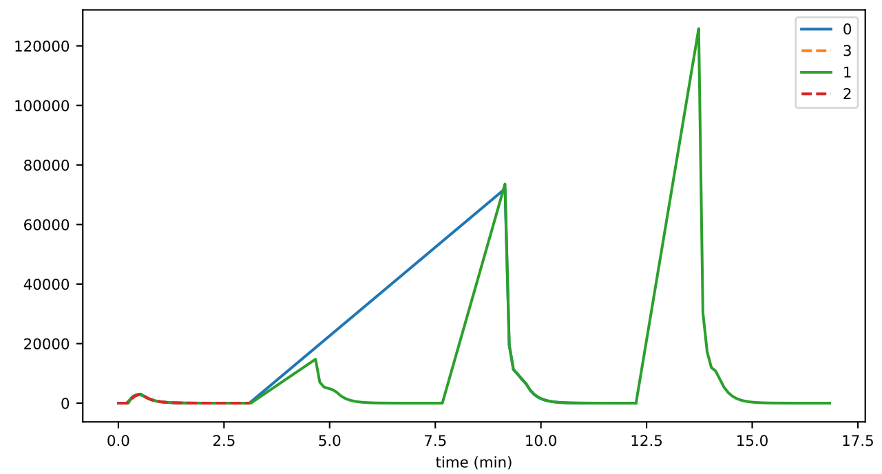
vmCreate
