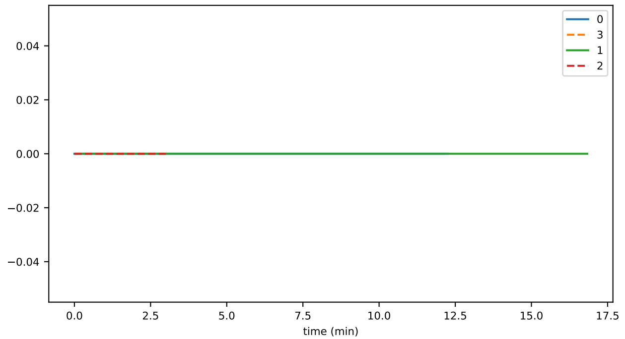
vmCreate
