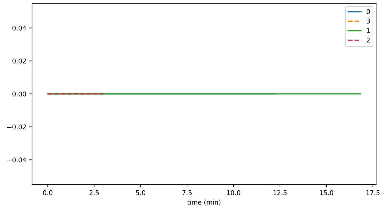
vmDelete
