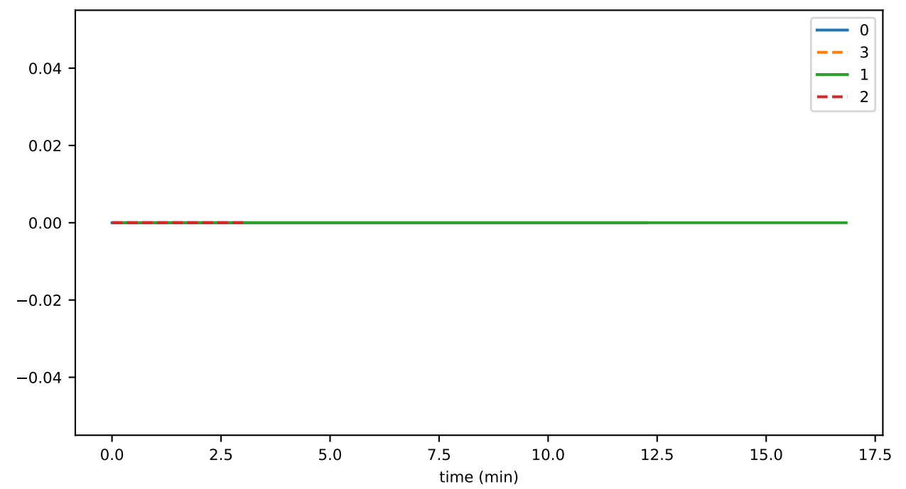
vmDelete
