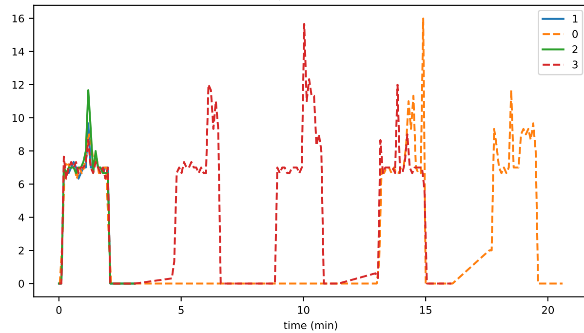
doNotSyncPlatformStatus
