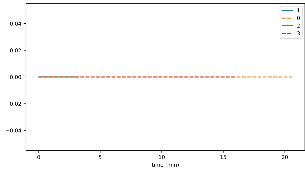
vmDelete
