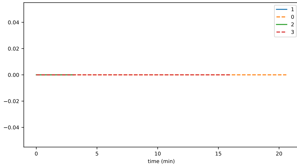
vmCreate
