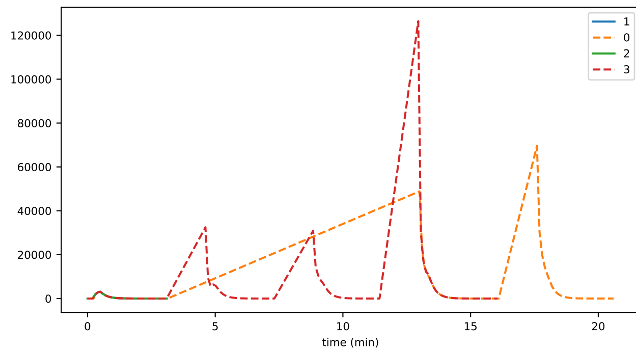
vmCreate
