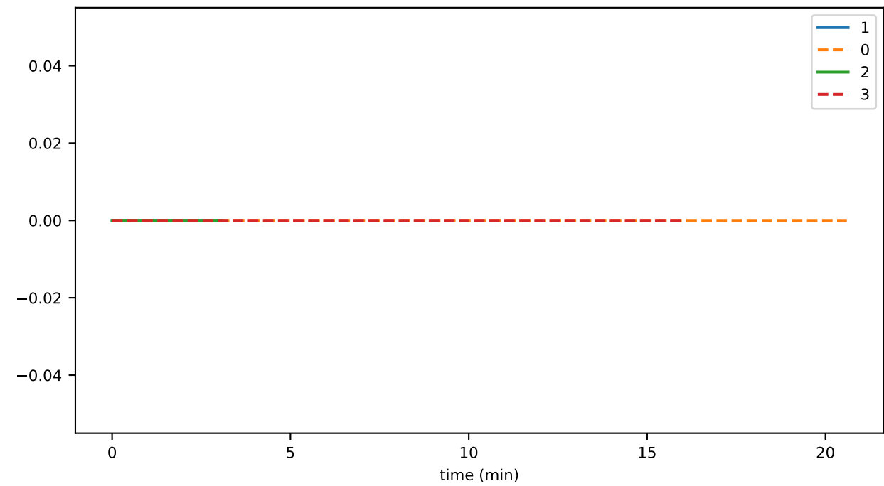
vmDelete
