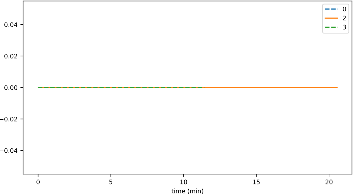
sync_phase_01_fraction_SENDING_EVENTS
