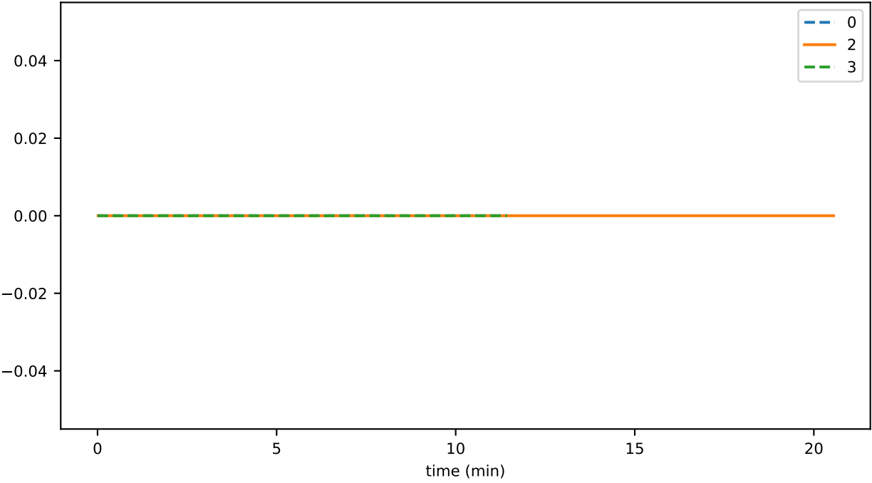
sync_phase_01_fraction_SELF_FALLEN_BEHIND
