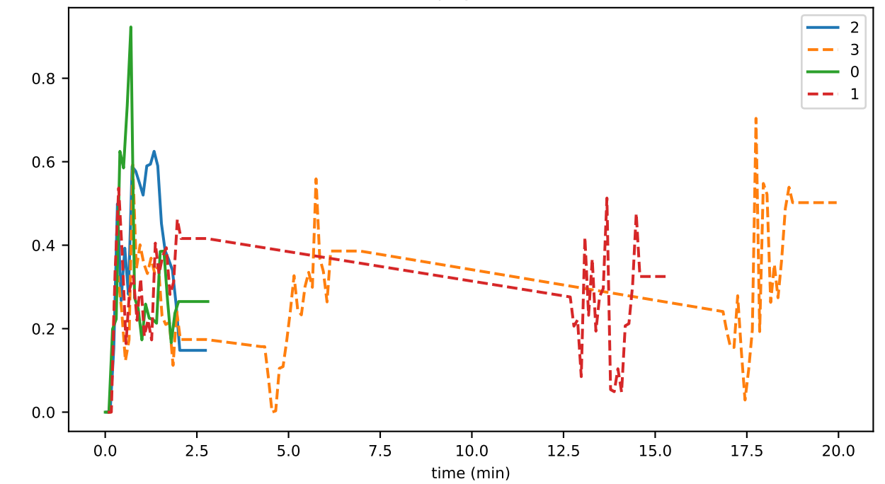
OrphanBuffer_unhandled_task_count
