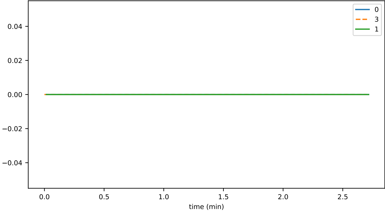
sync_phase_02_fraction_SENDING_EVENTS
