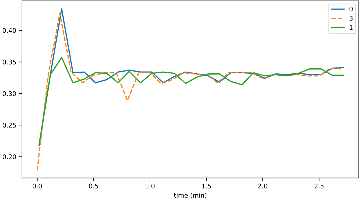
sync_phase_02_fraction_SENDING_EVENTS
