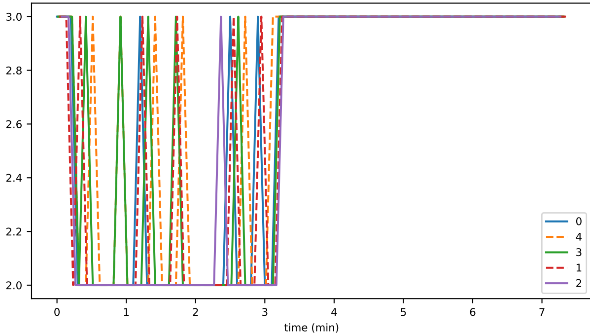
vmap_lifecycle_pipelineSize_state
