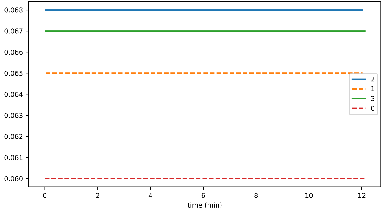
memFree
