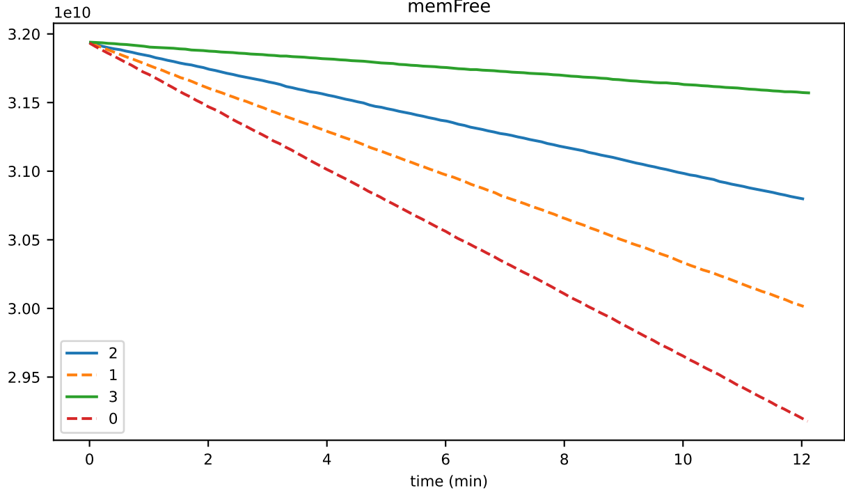
memFree
