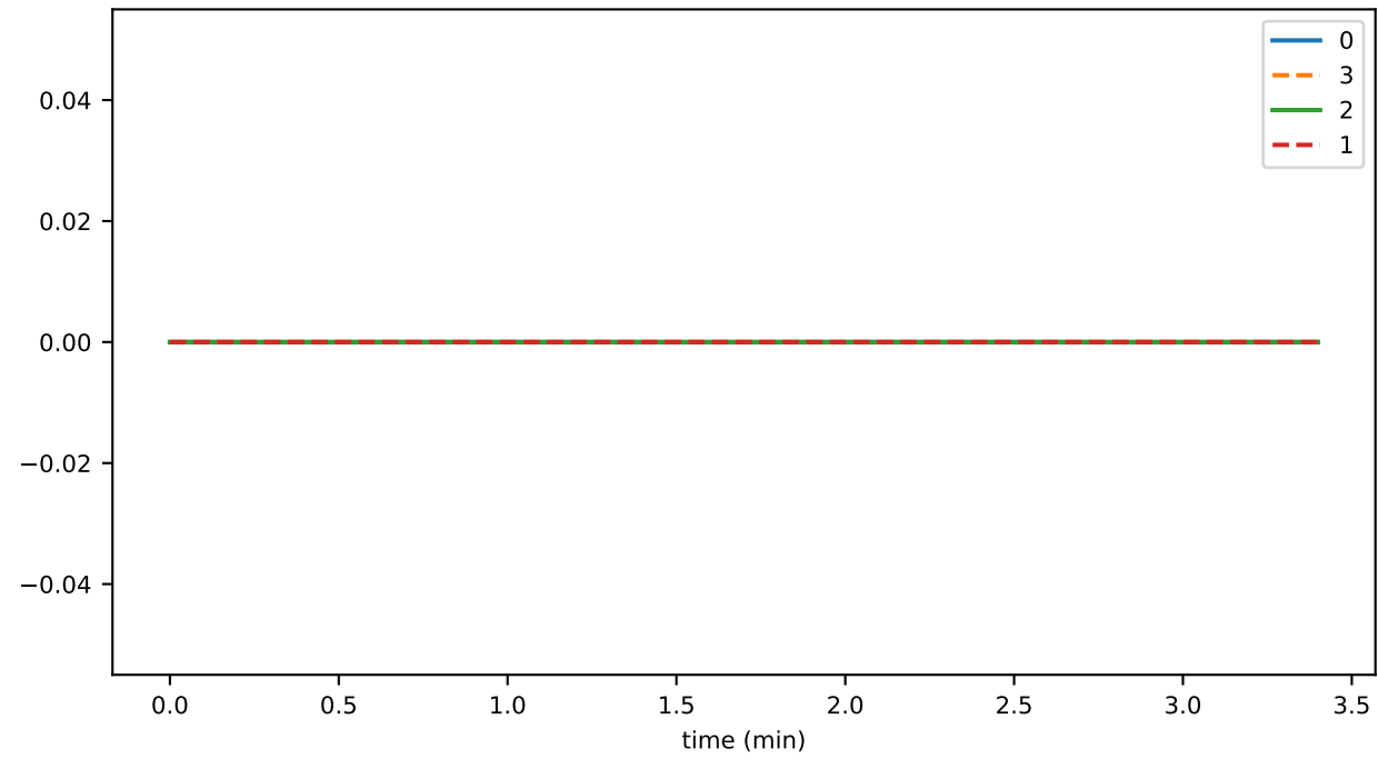
opportunitiesToInitiateSync_per_sec
