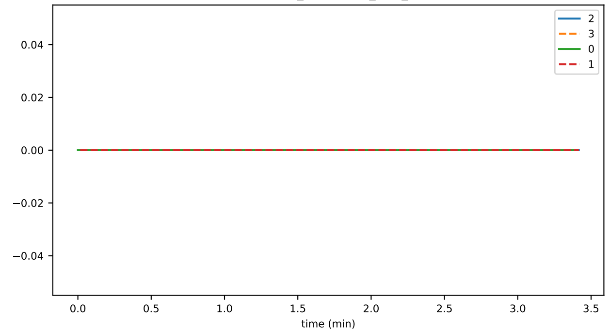
OrphanBuffer_unhandled_task_count
