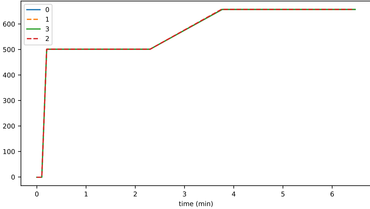
preconsensusEventFileYoungestIdentifier
