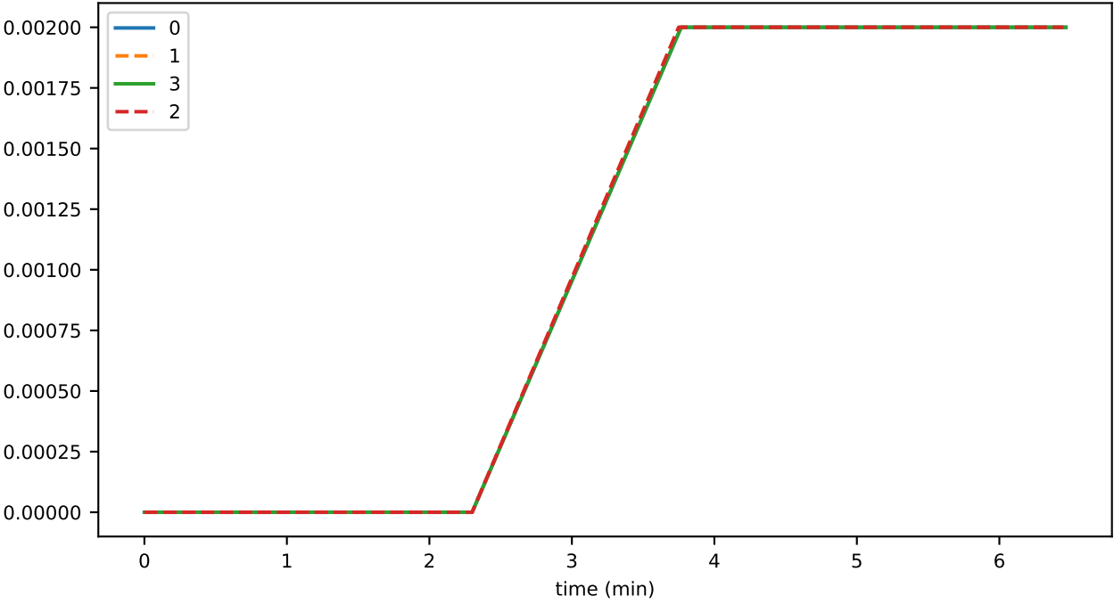
preconsensusEventFileTotalSizeGB
