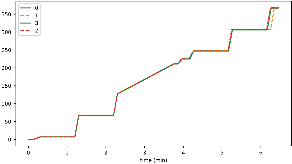
preconsensusEventFileTotalSizeGB
