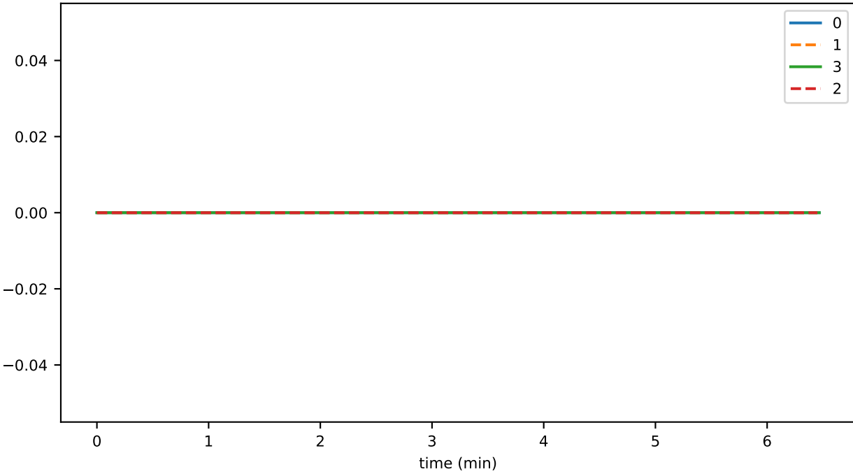
preconsensusEventFileYoungestIdentifier
