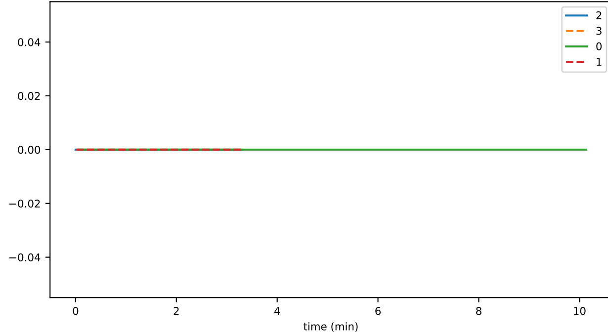
BranchDetector_unhandled_task_count
