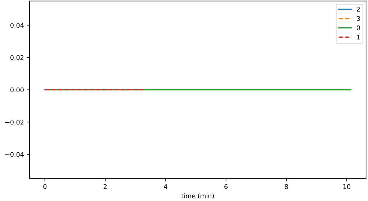
branchingEvents
