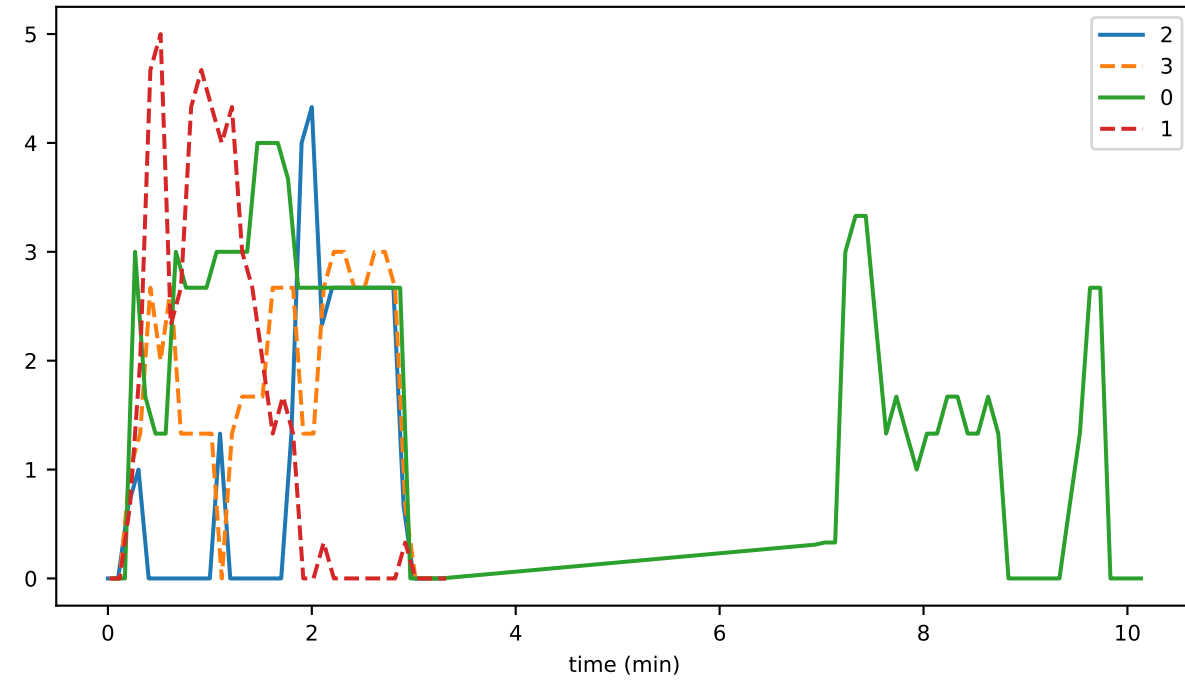
BranchDetector_unhandled_task_count
