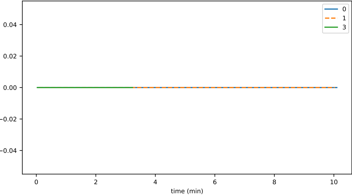
sync_phase_02_fraction_SENDING_EVENTS
