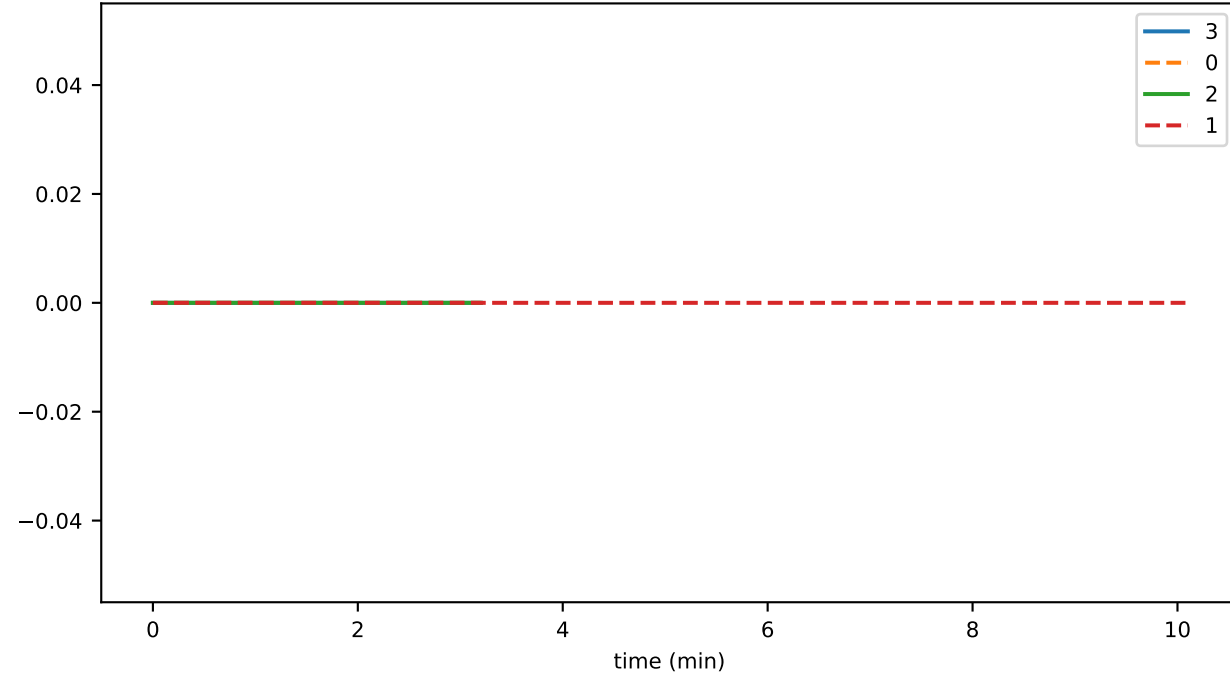
totalNeverSignedStates
