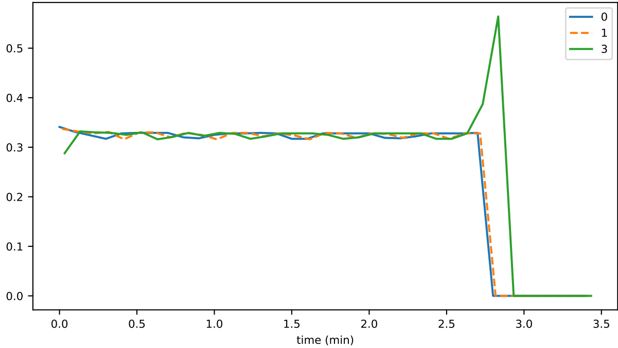
sync_phase_02_fraction_SENDING_EVENTS
