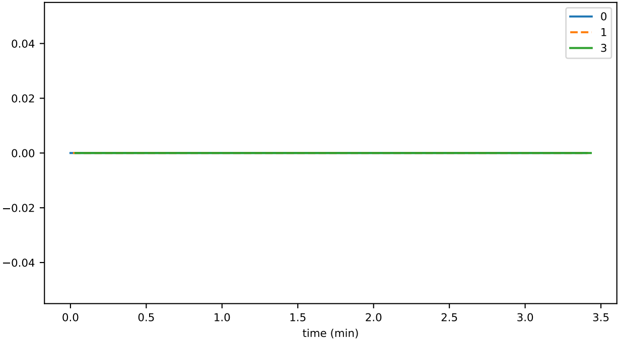
sync_phase_02_fraction_SELF_FALLEN_BEHIND
