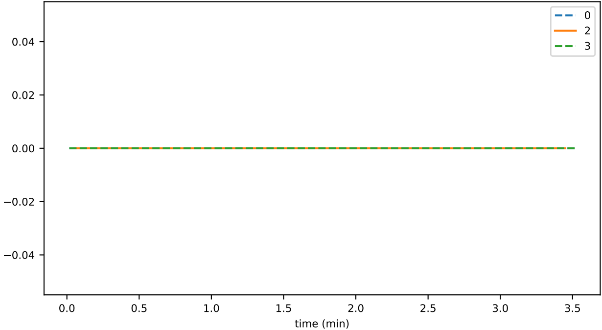
sync_phase_01_fraction_SENDING_EVENTS
