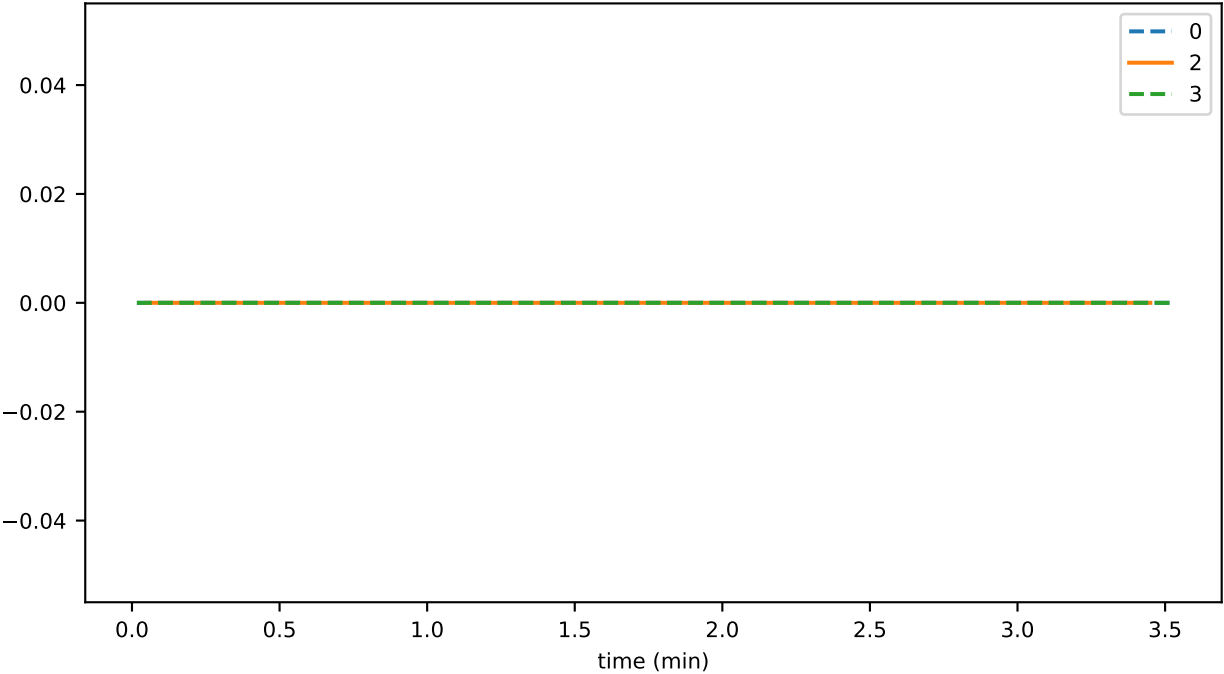
sync_phase_01_fraction_SELF_FALLEN_BEHIND
