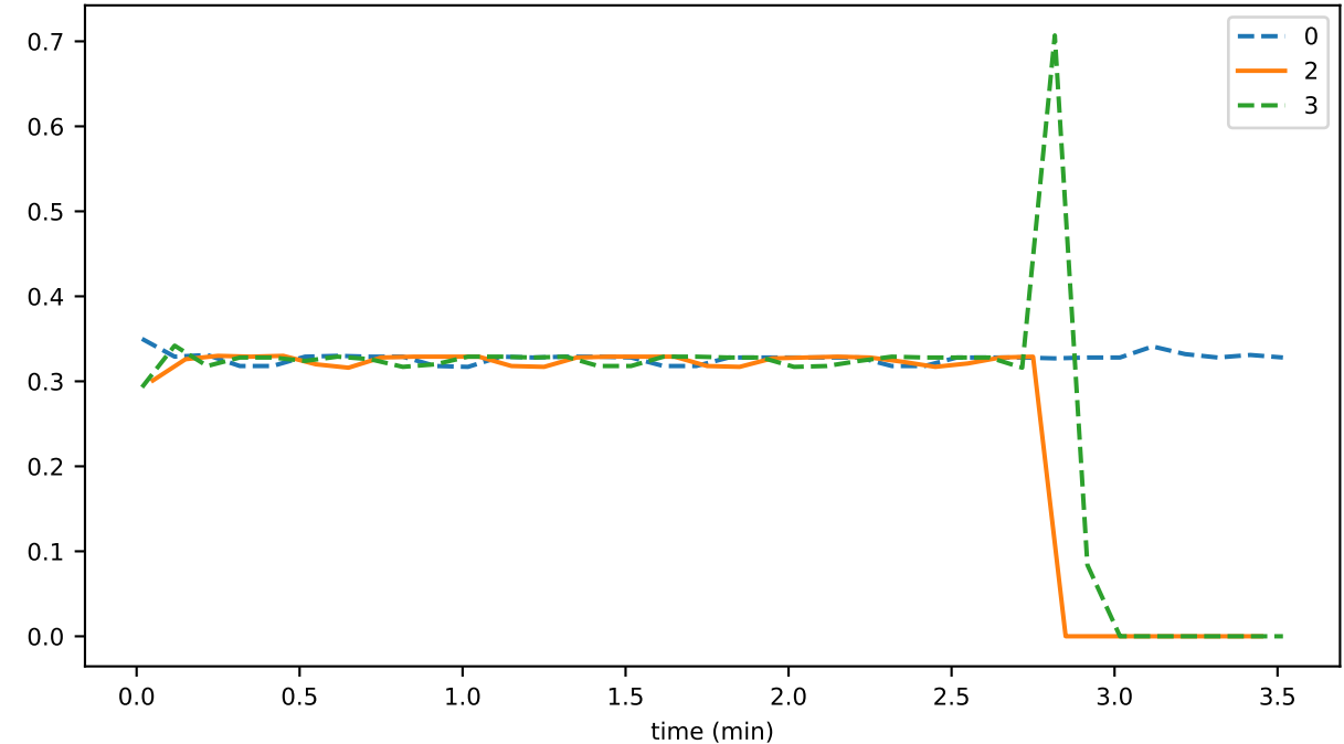
sync_phase_01_fraction_SENDING_EVENTS
