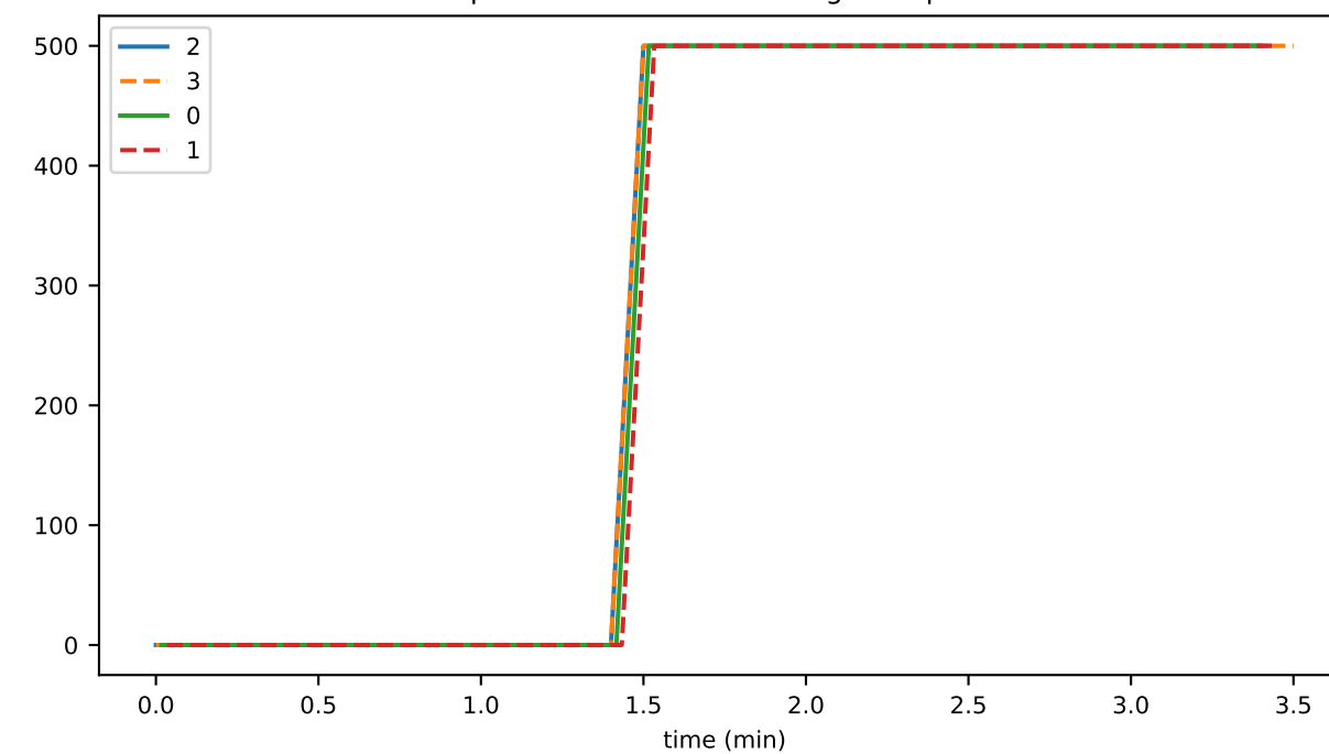
preconsensusEventAverageFileSpan
