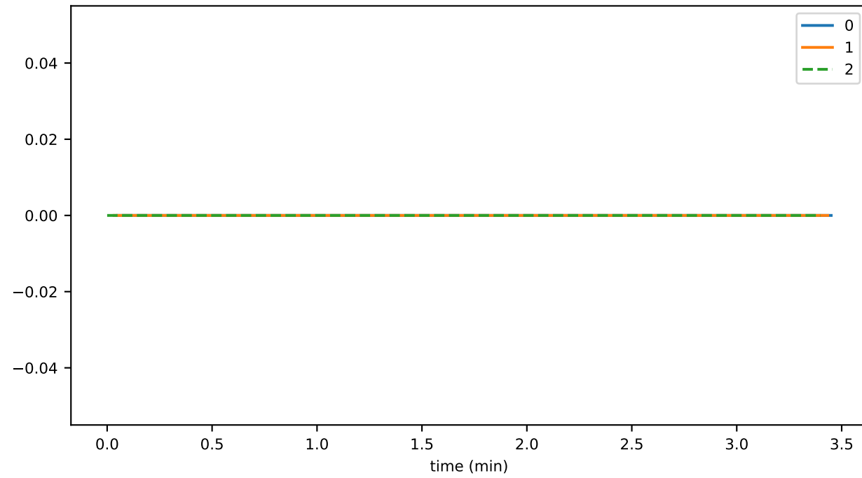
sync_phase_03_fraction_SENDING_EVENTS
