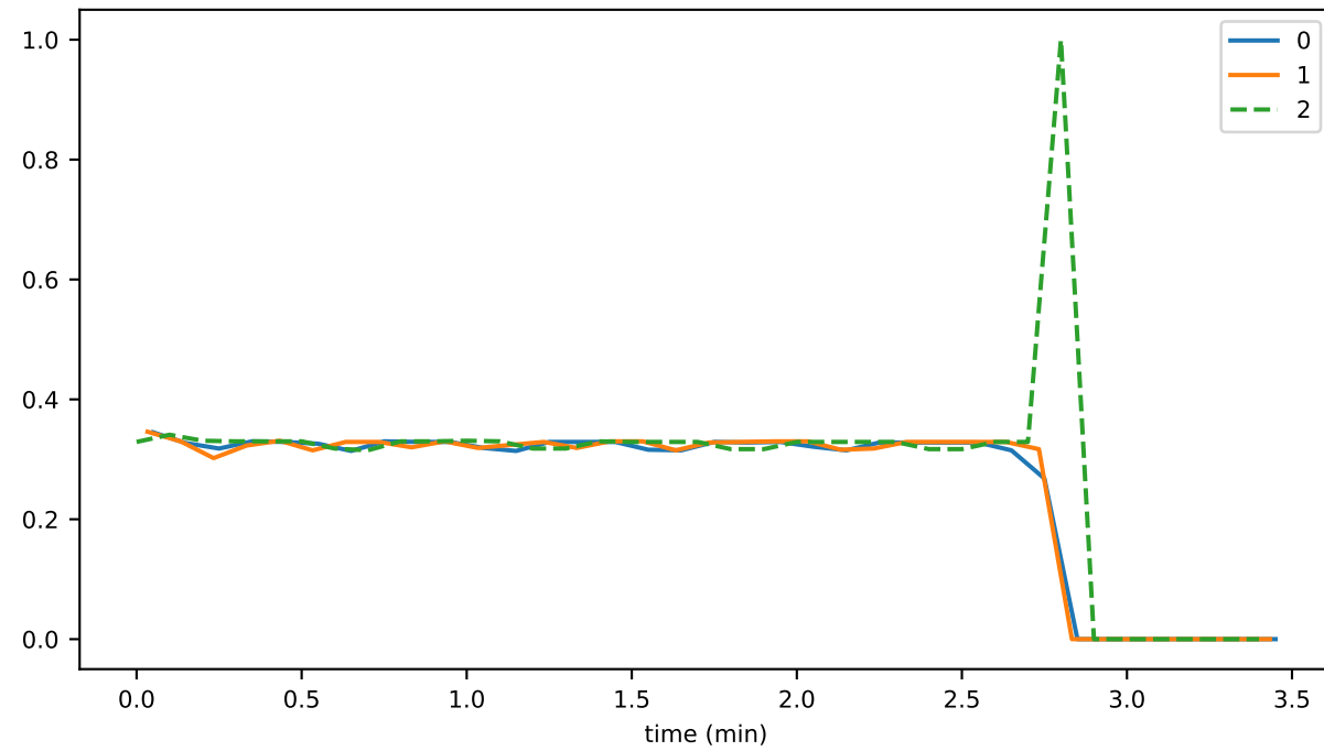
sync_phase_03_fraction_SENDING_EVENTS
