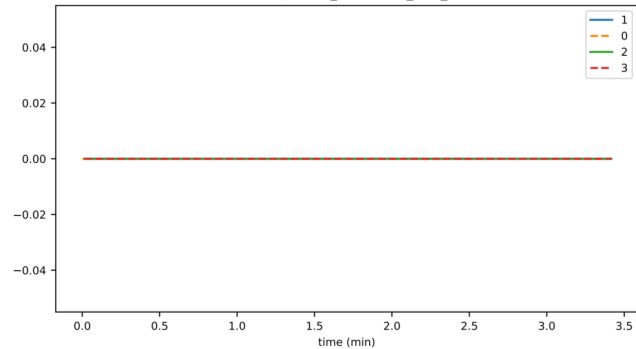
eventRecRate
