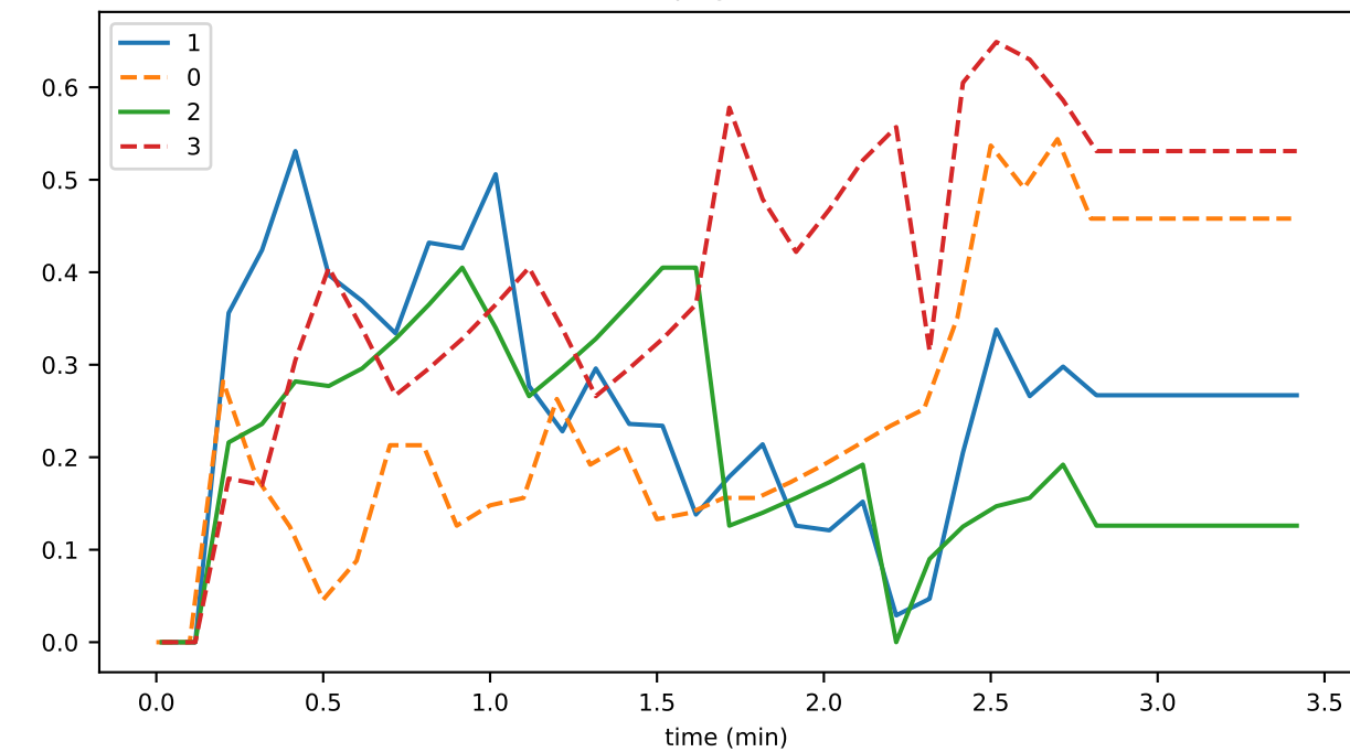
OrphanBuffer_unhandled_task_count
