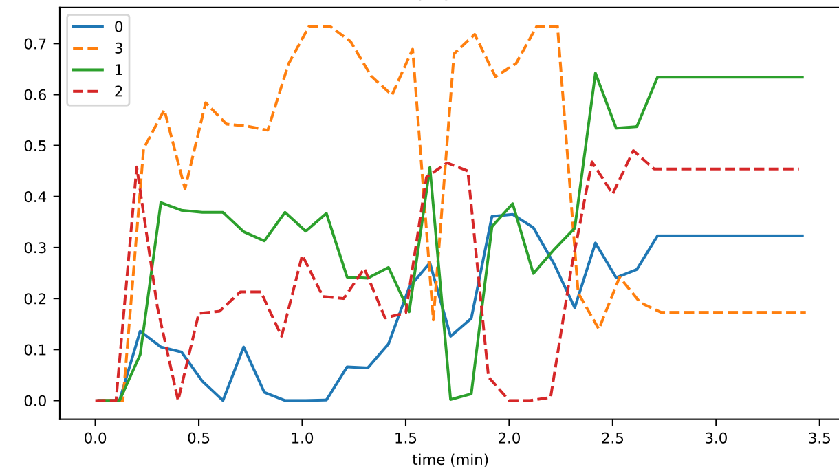
OrphanBuffer_unhandled_task_count
