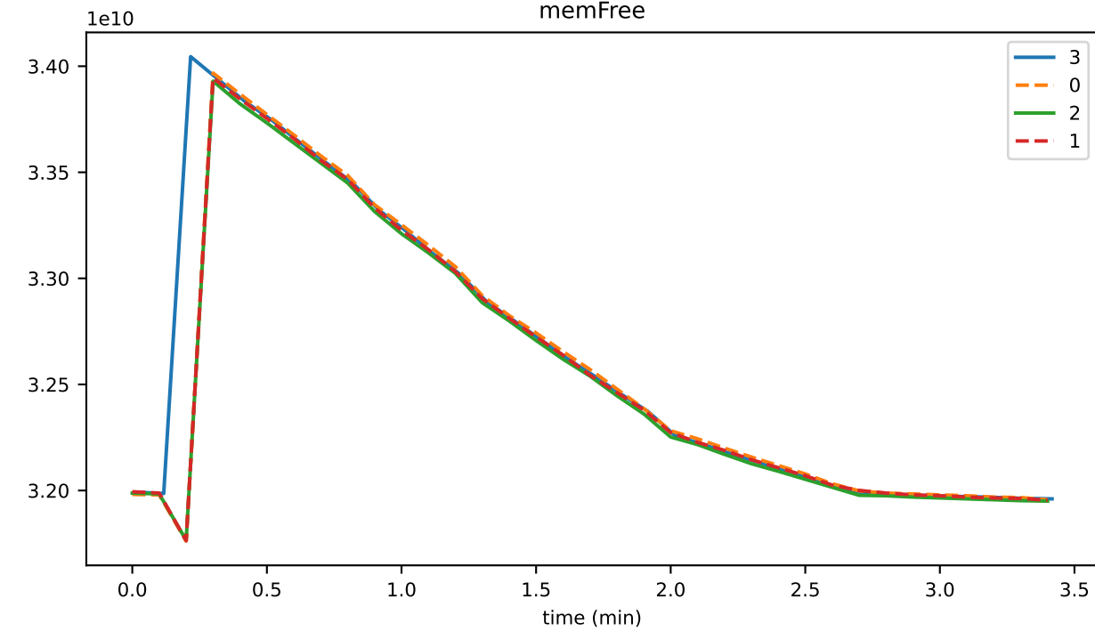
memFree
