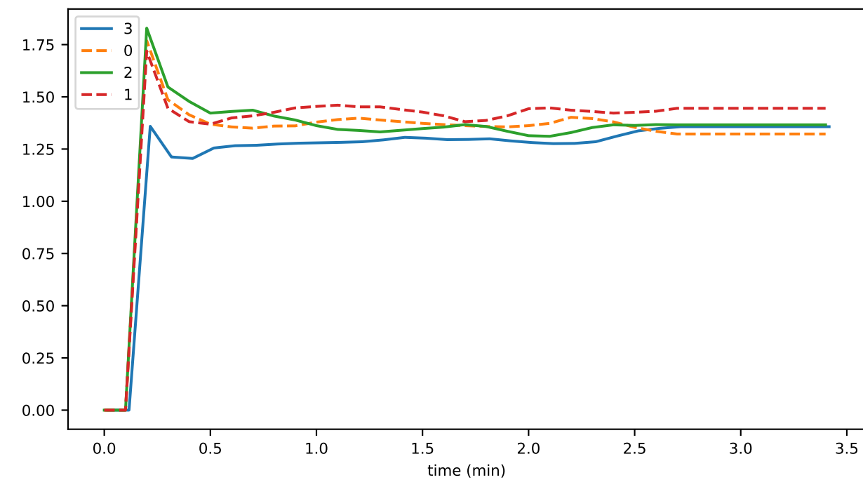
memFree
