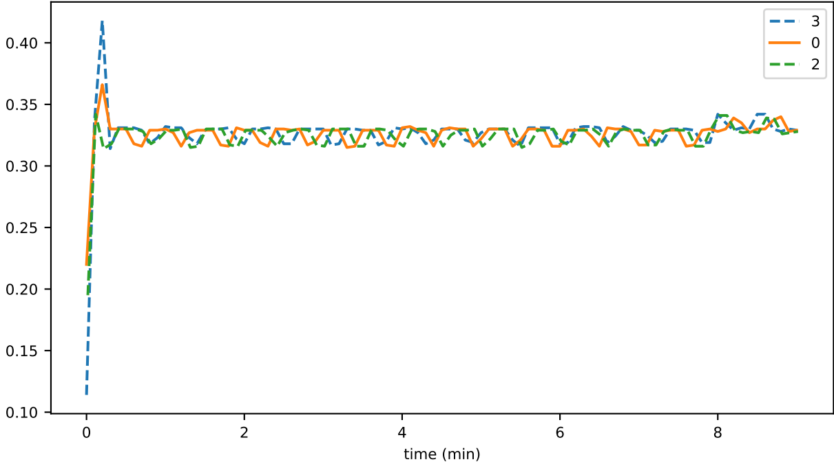
sync_phase_01_fraction_SENDING_EVENTS
