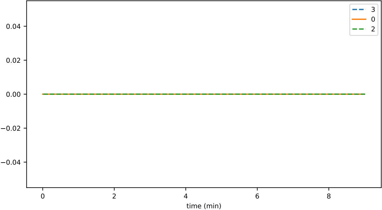
sync_phase_01_fraction_SELF_FALLEN_BEHIND
