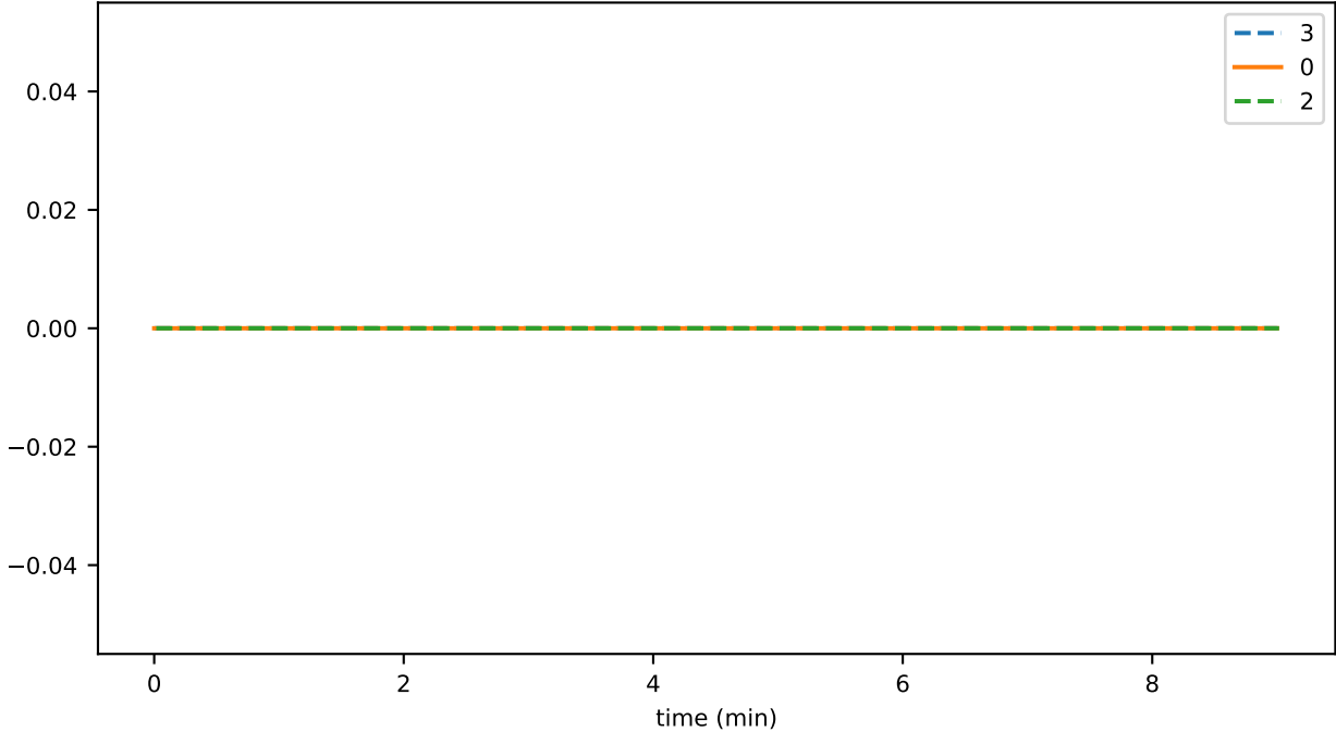
sync_phase_01_fraction_SENDING_EVENTS
