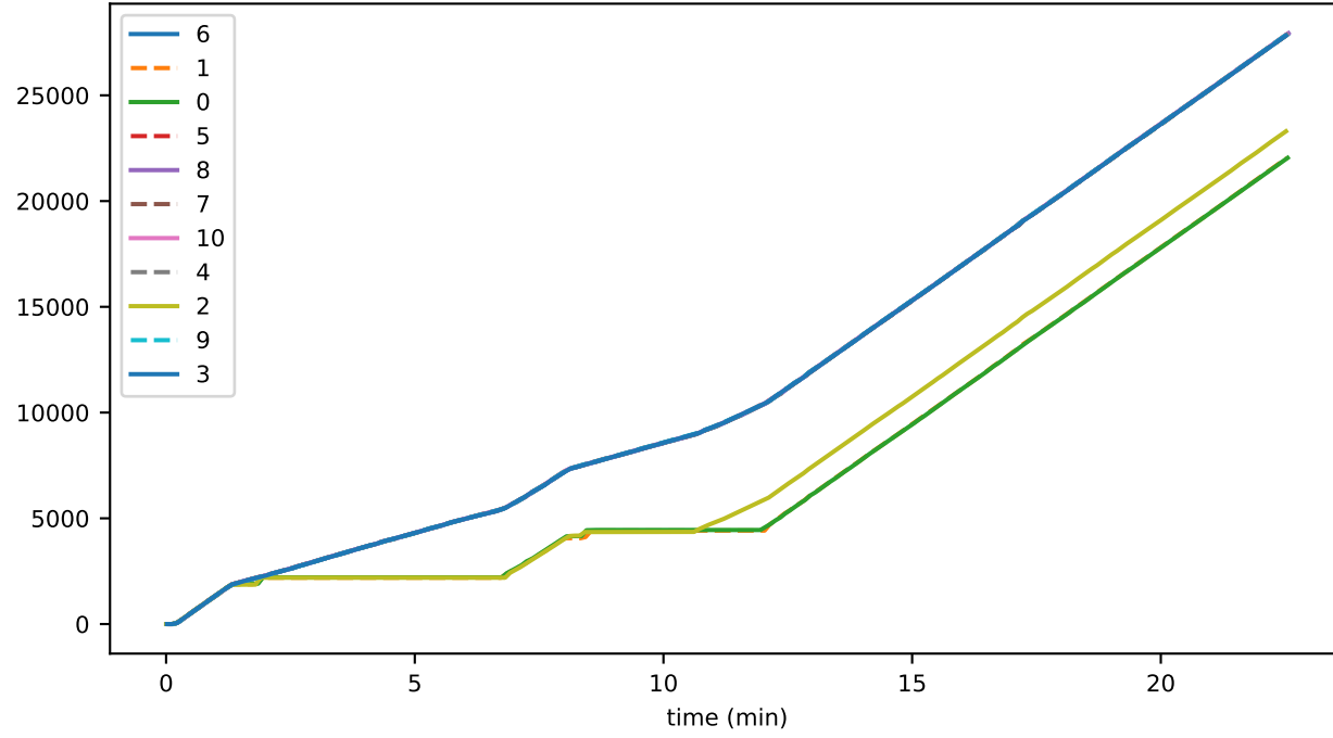
roundIncEqParents
