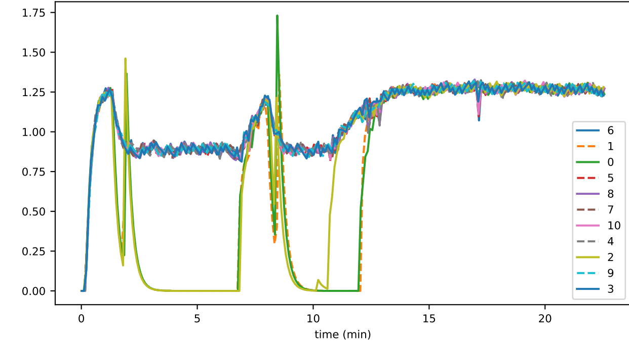
rounds_per_sec
