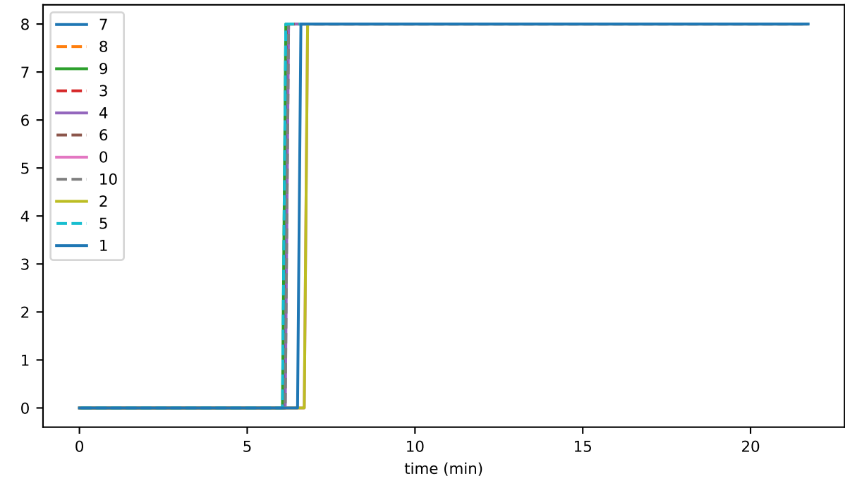
ds_reads_leafKeys_accounts
