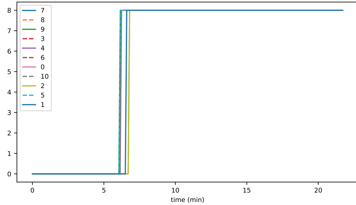
ds_reads_hashes_accounts
