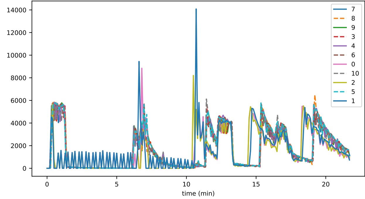
ds_reads_leafKeys_accounts
