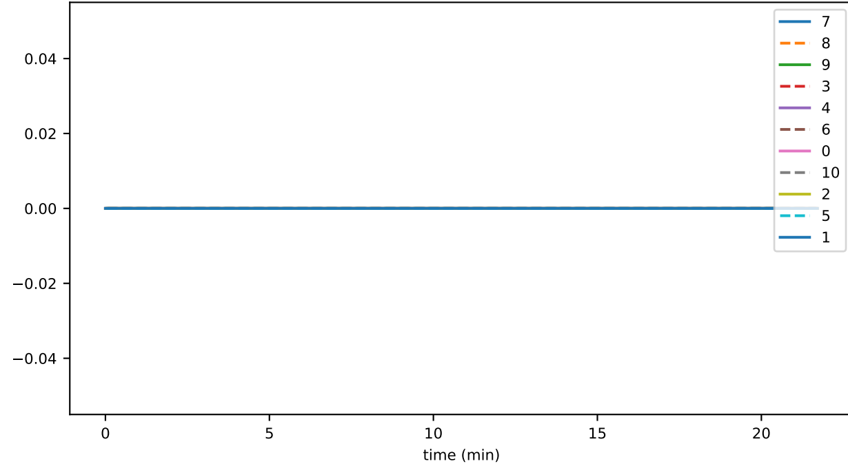
ds_reads_hashes_accounts
