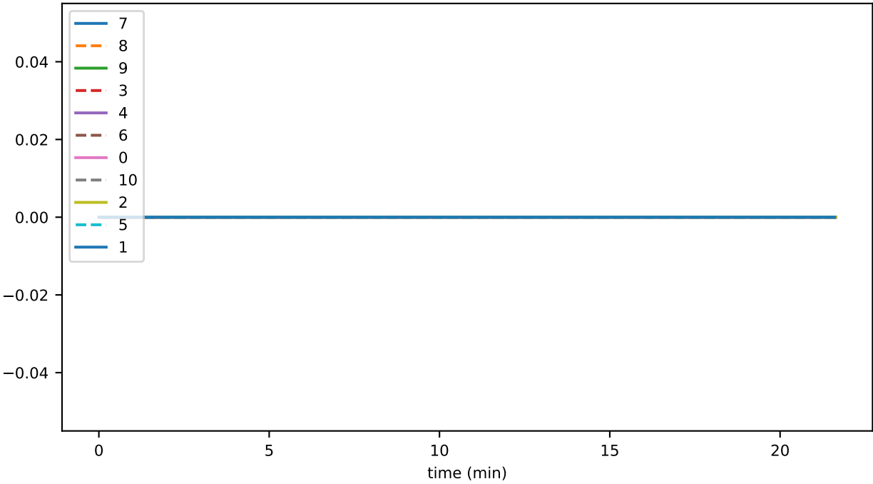
ds_compactions_level_1_hashesSavedSpaceMb_accounts
