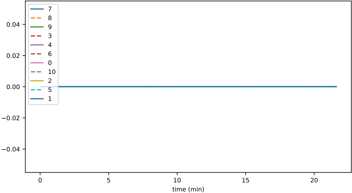
branchingNodeCount
