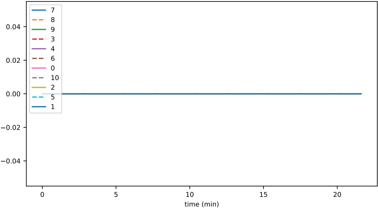
ds_compactions_level_0_leavesTimeMs_accounts
