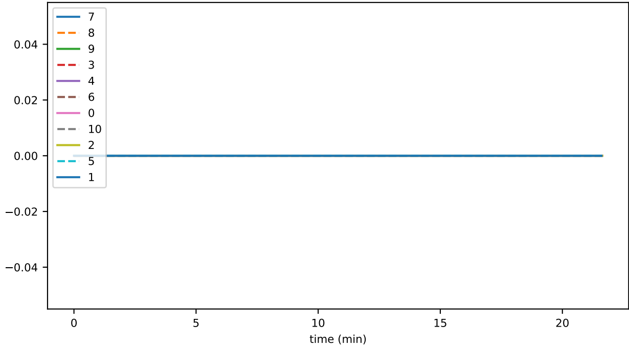
branchingWeightFraction
