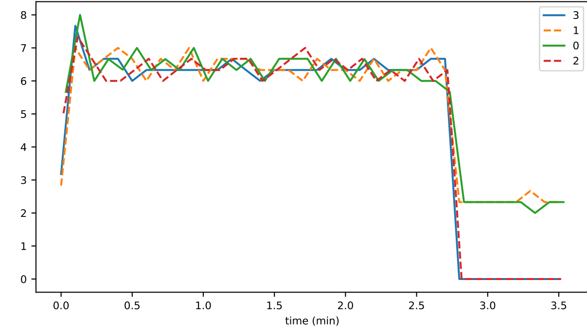
opportunitiesToInitiateSync_per_sec
