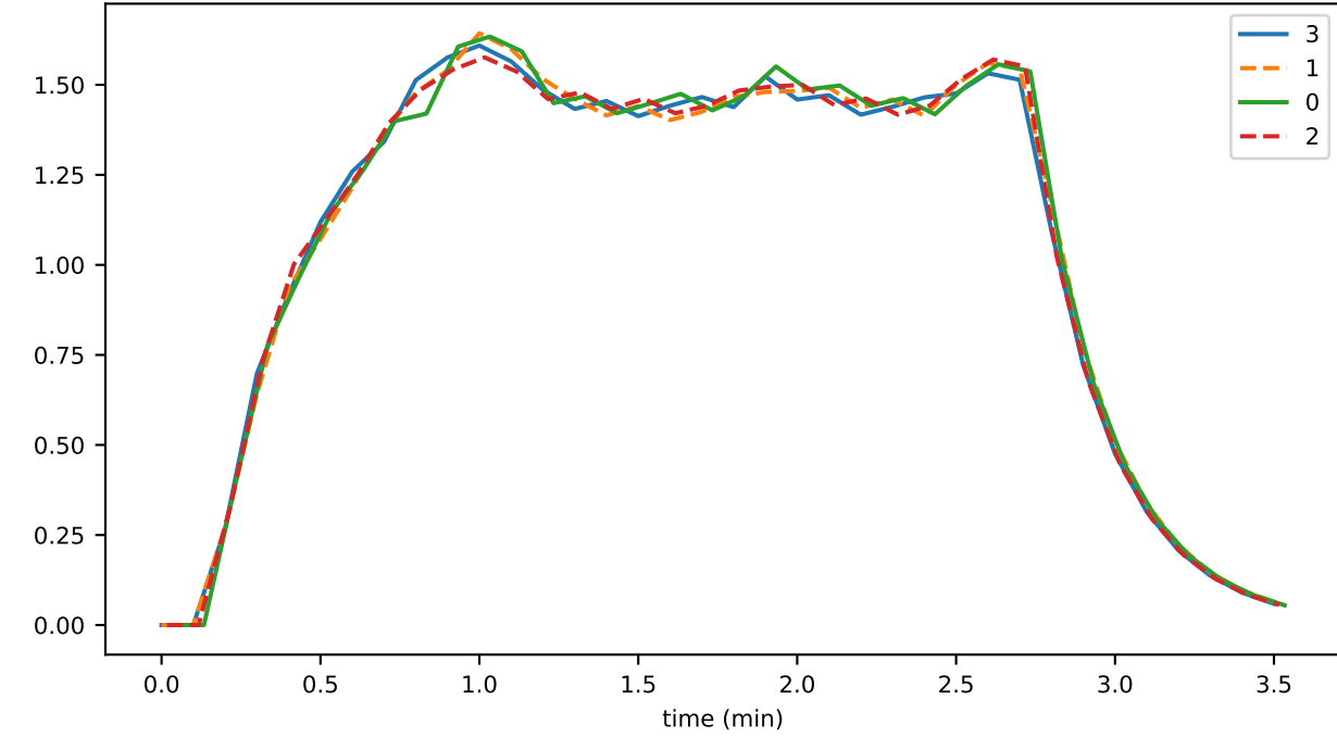
rounds_per_sec
