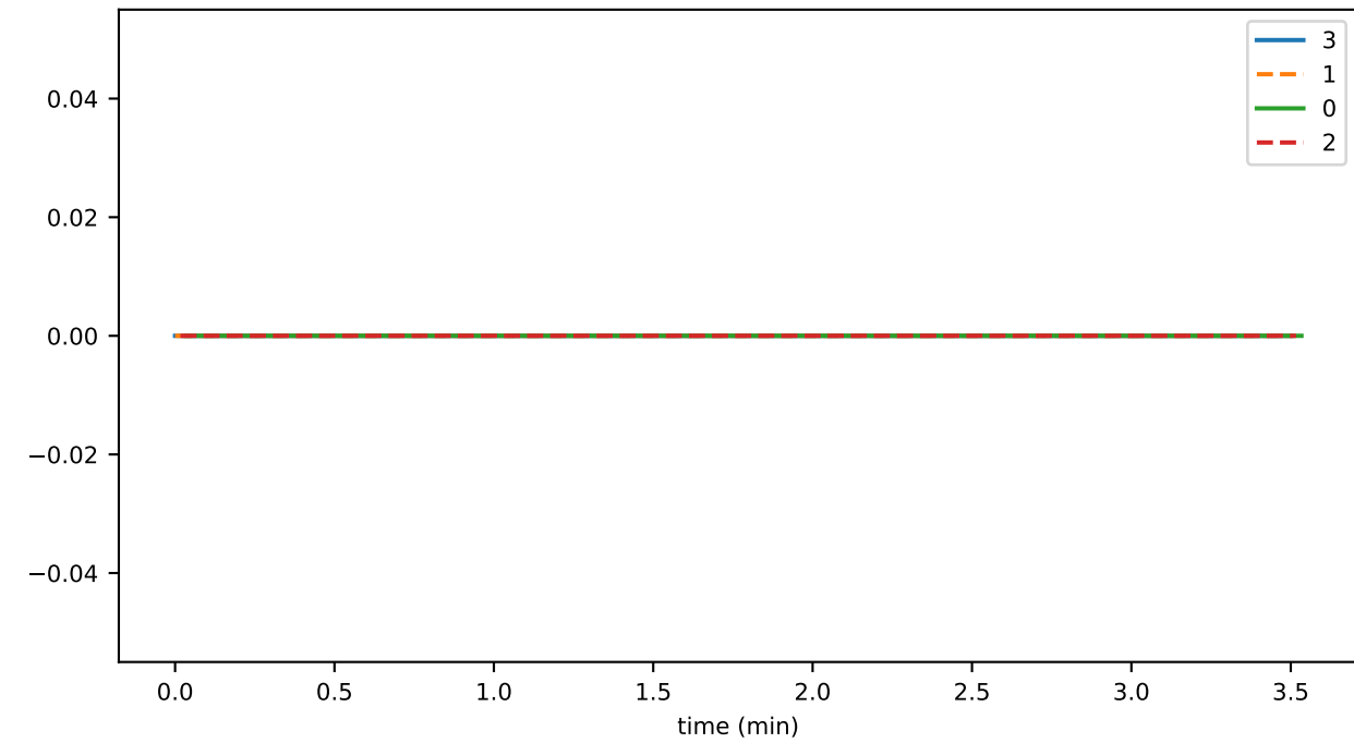
rounds_per_sec
