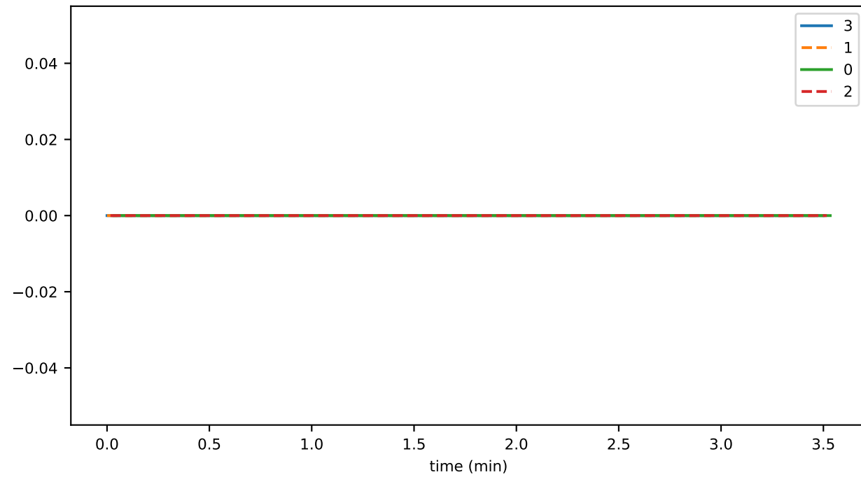
opAgeDiff
