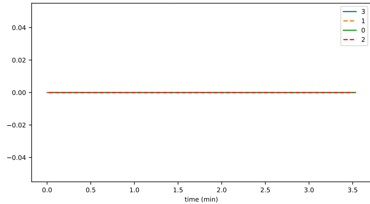
SigWrkTime
