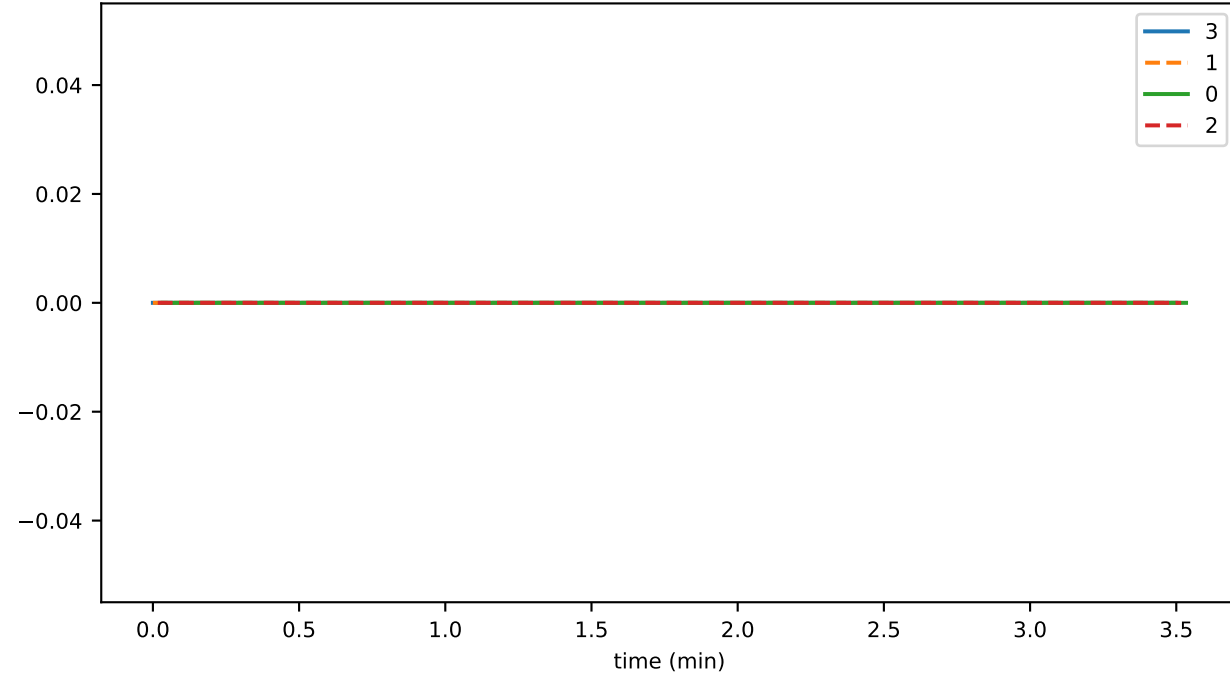
opAgeDiff
