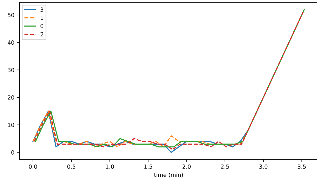
opportunitiesToInitiateSync_per_sec
