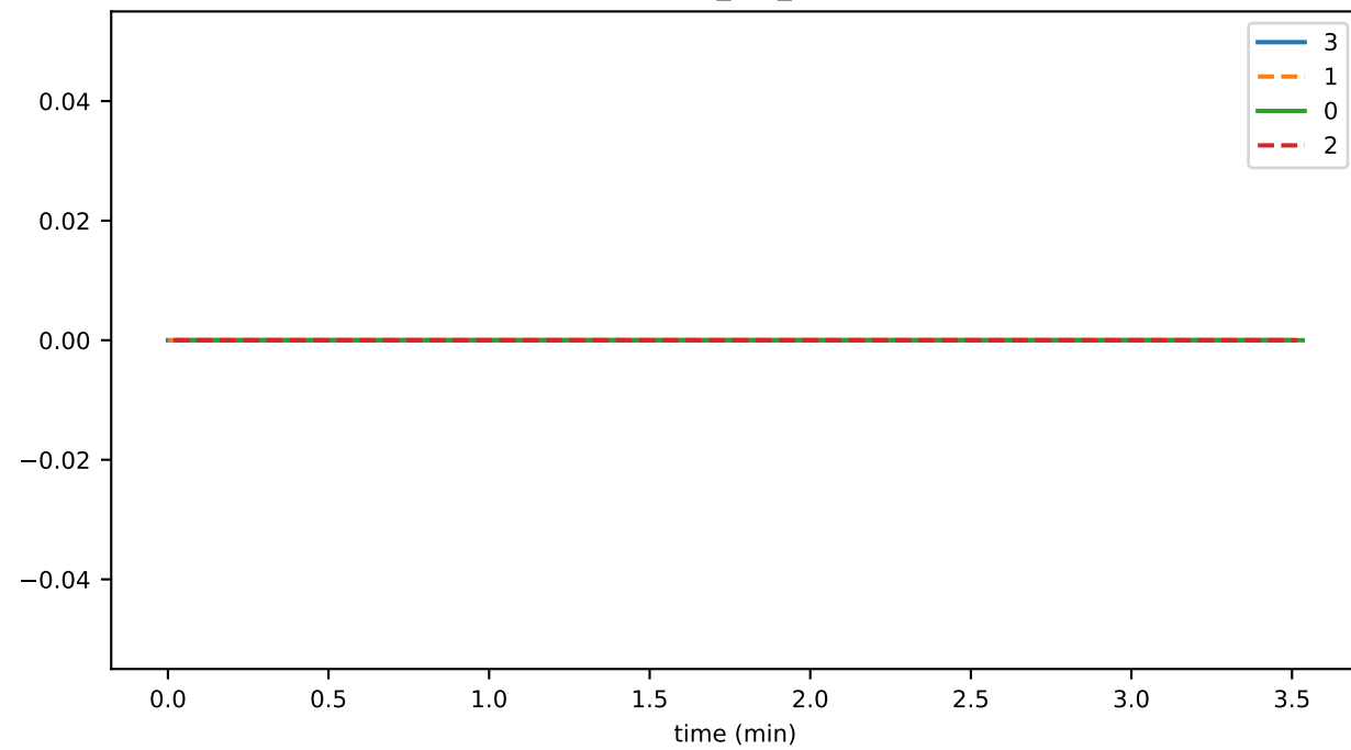
SigVal_per_sec
