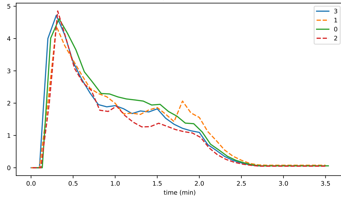
SigVal_per_sec
