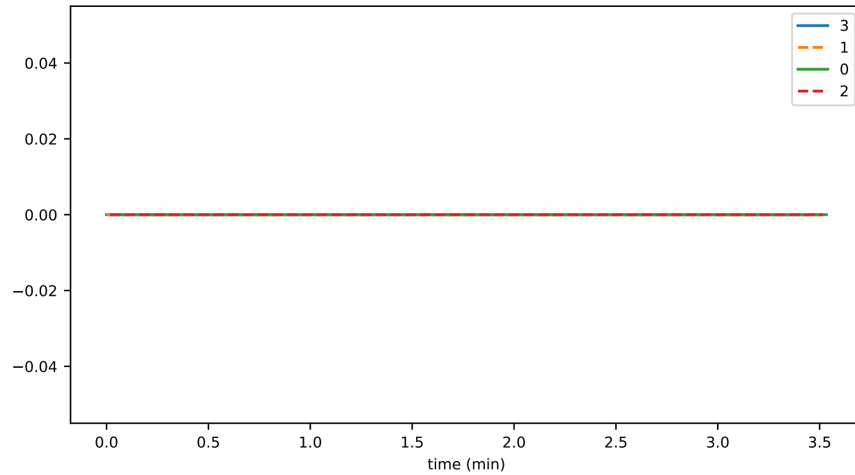
roundIncEqParents
