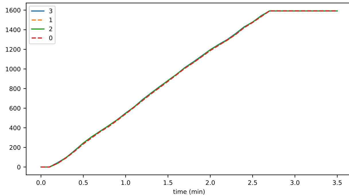
roundIncEqParents
