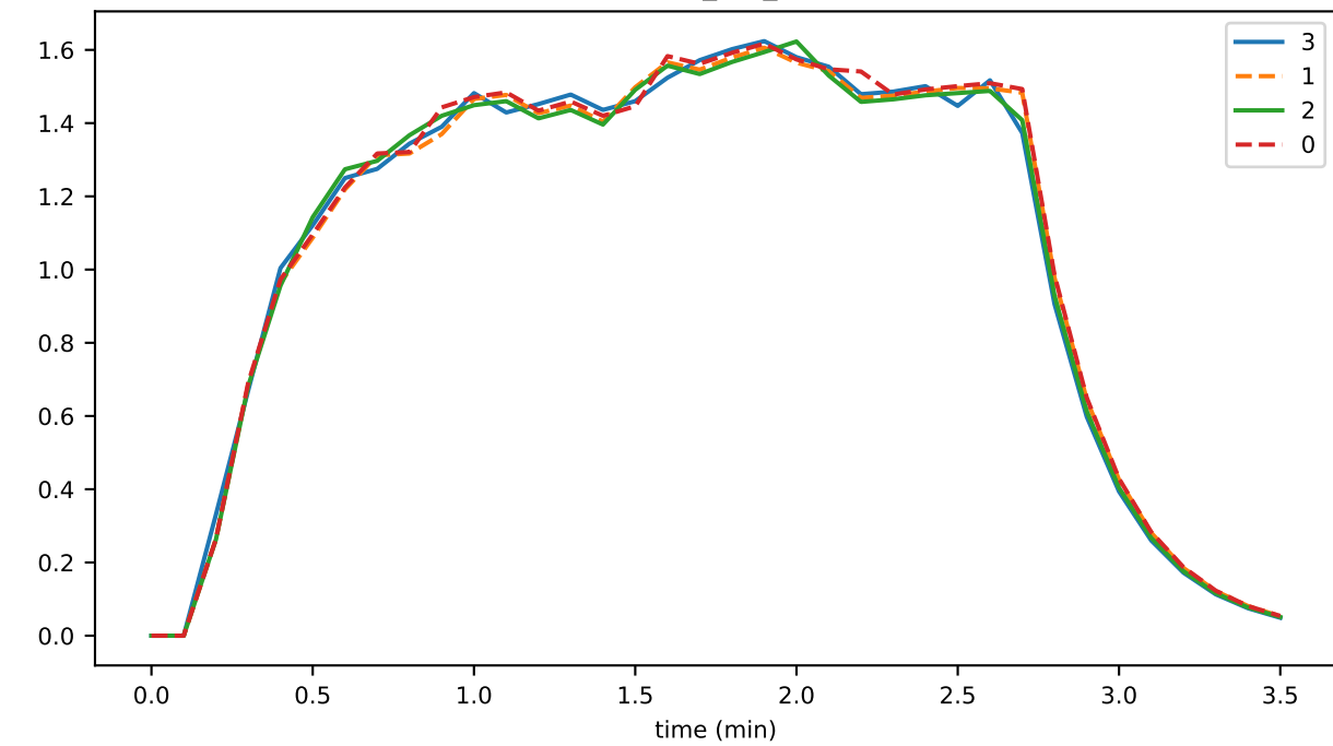
rounds_per_sec
