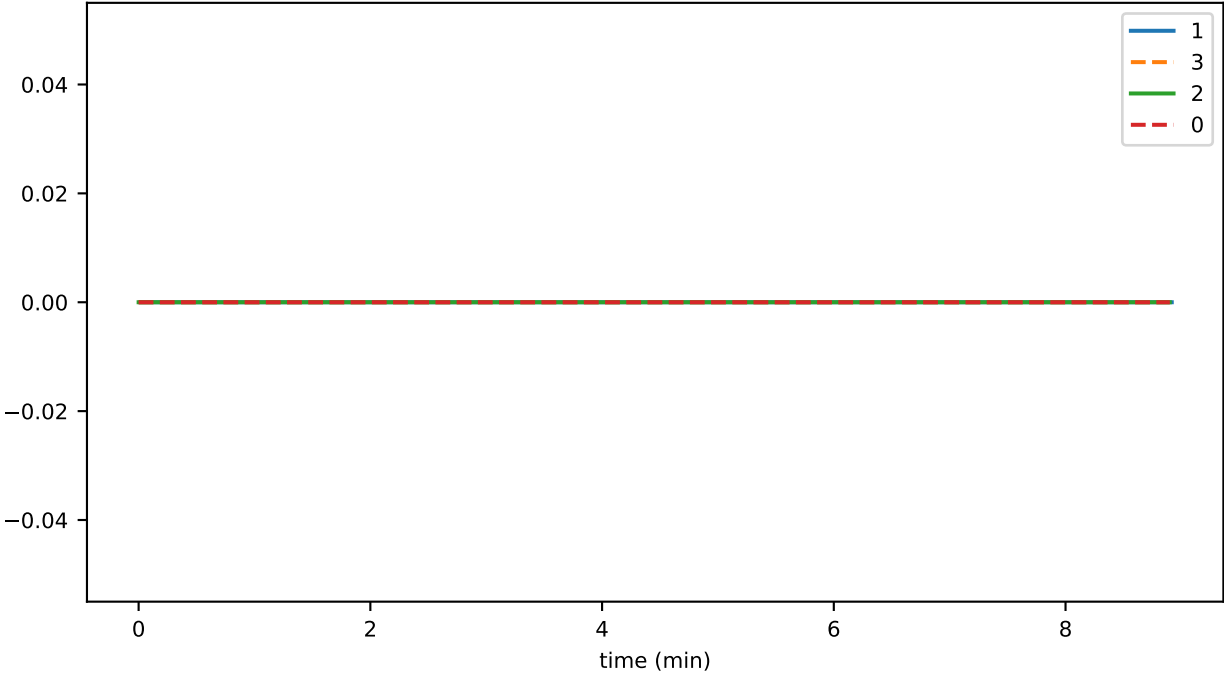
ds_compactions_level_2_hashesTimeMs_accounts
