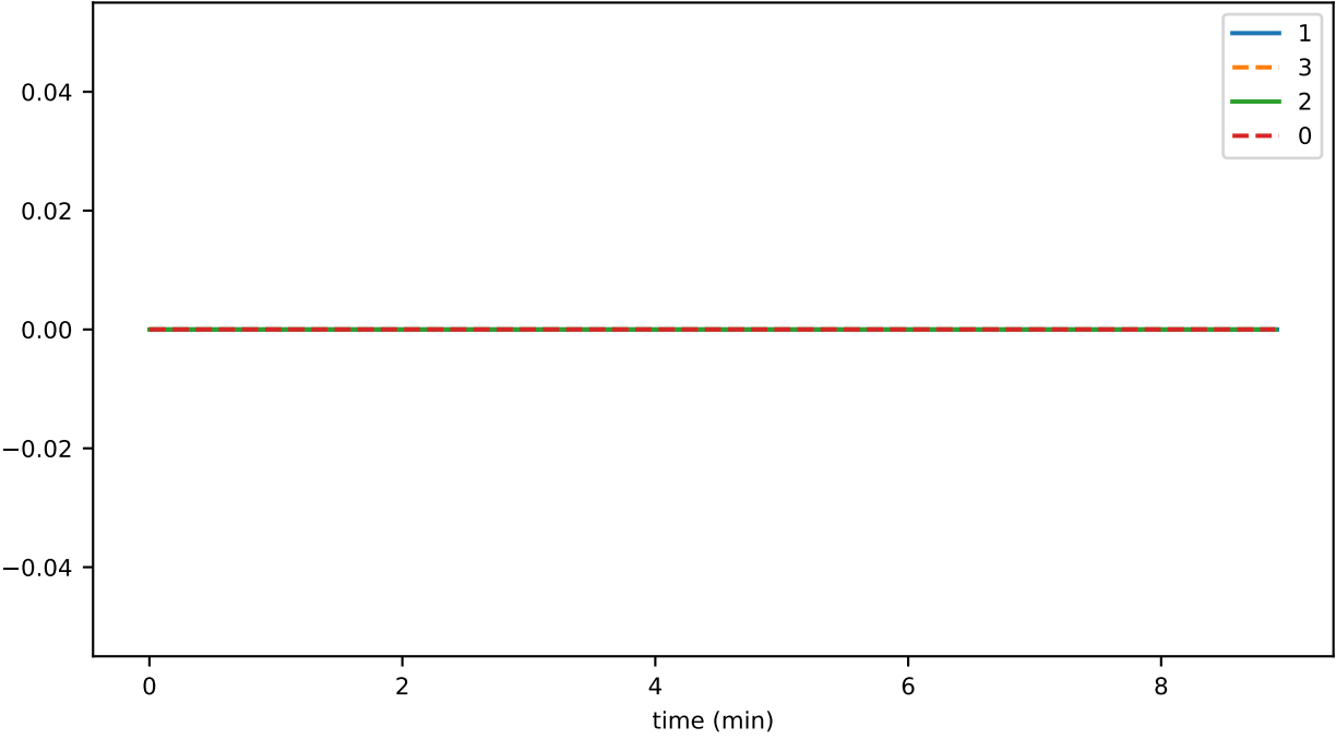
ds_compactions_level_2_hashesSavedSpaceMb_accounts
