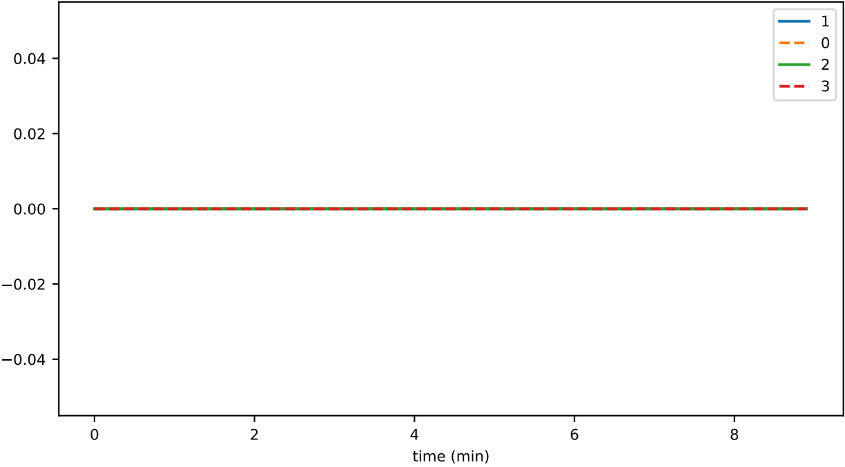
ds_files_hashesStoreFileCount_accounts
