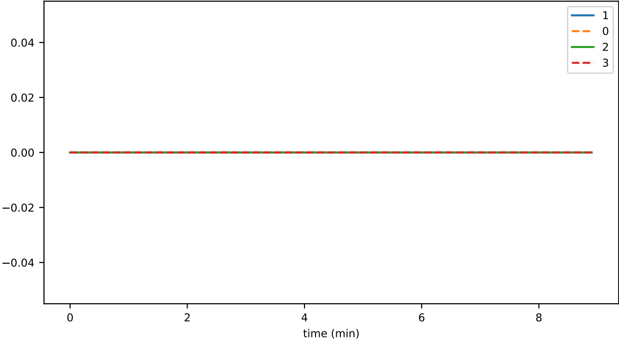
ds_files_hashesStoreFileSizeMb_accounts
