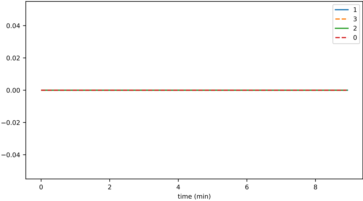
ds_compactions_level_3_leafKeysTimeMs_accounts
