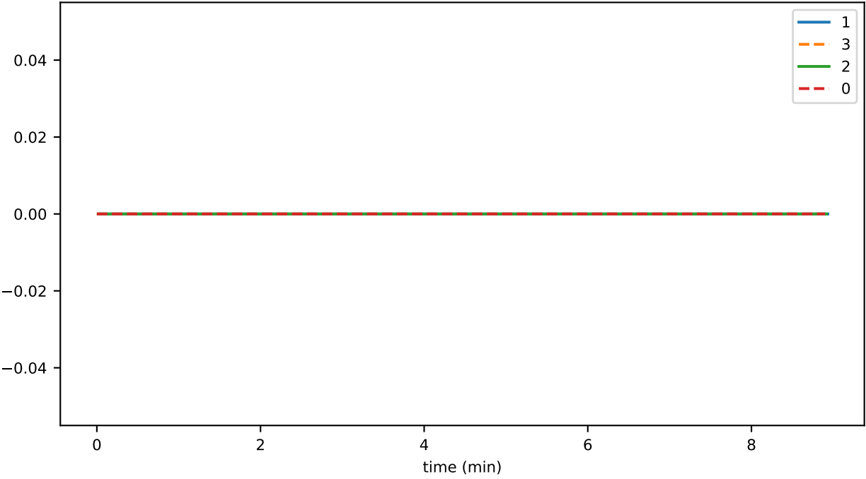
ds_compactions_level_3_leafKeysSavedSpaceMb_accounts
