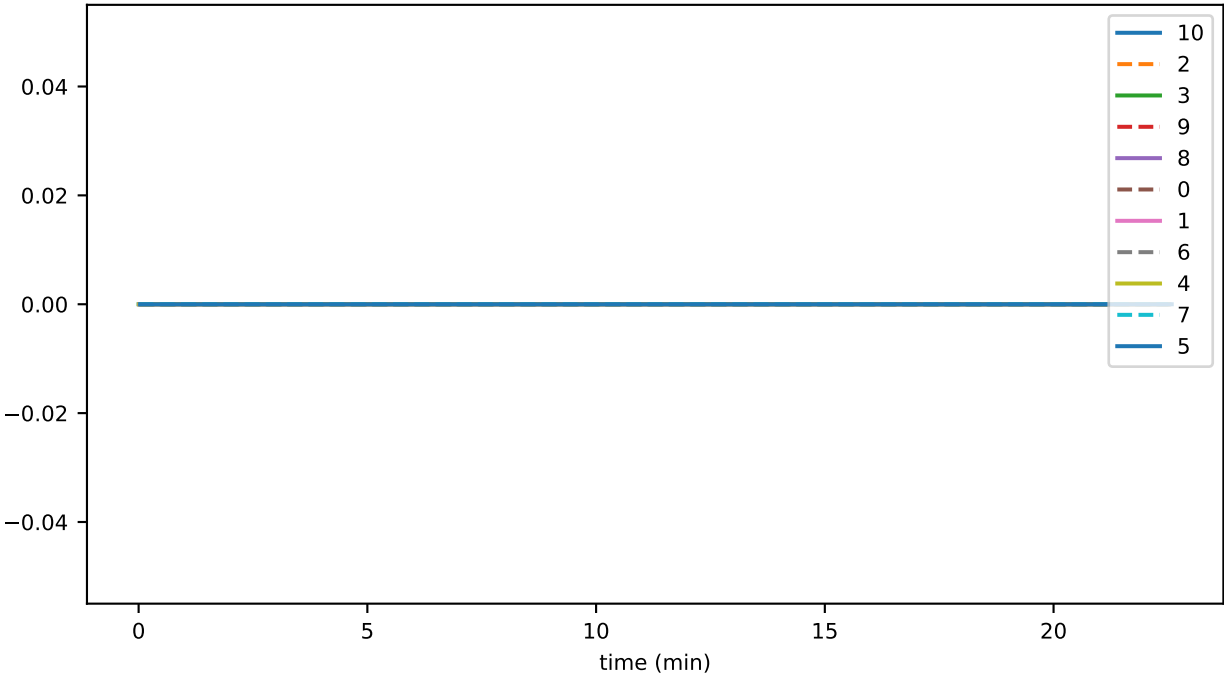
ds_files_level_3_leafKeysFileSizeByLevelMb_accounts
