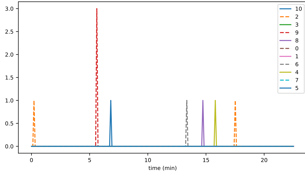
eventRecRate
