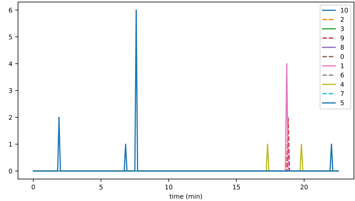
events_per_sec
