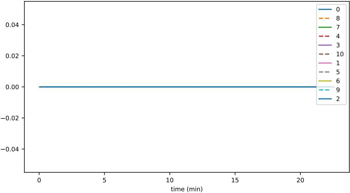
vmap_lifecycle_flushCount_accounts
