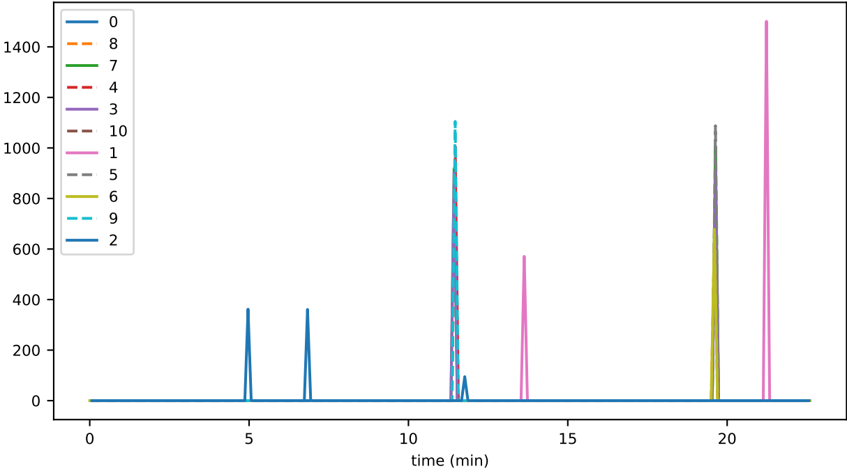
vmap_lifecycle_flushDurationMs_accounts
