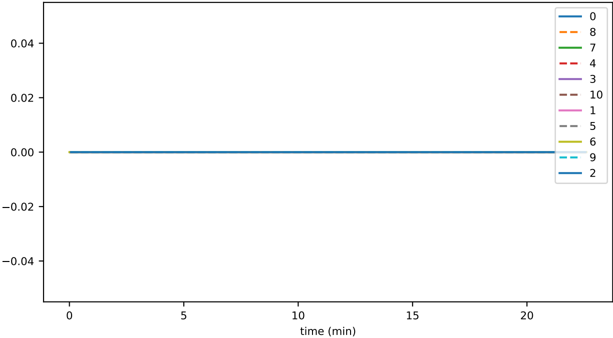
vmap_lifecycle_flushDurationMs_accounts
