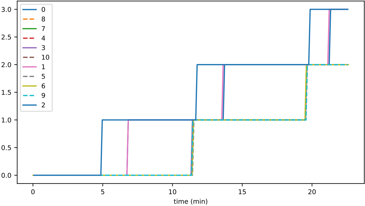
vmap_lifecycle_flushCount_accounts
