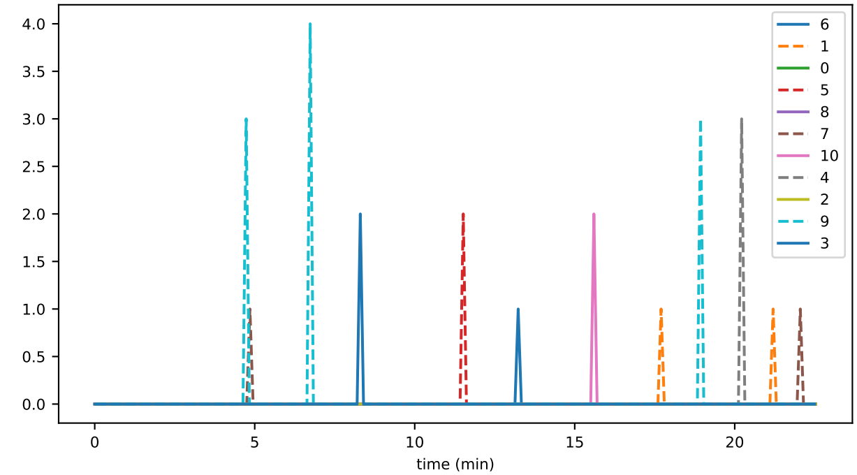
events_per_sec
