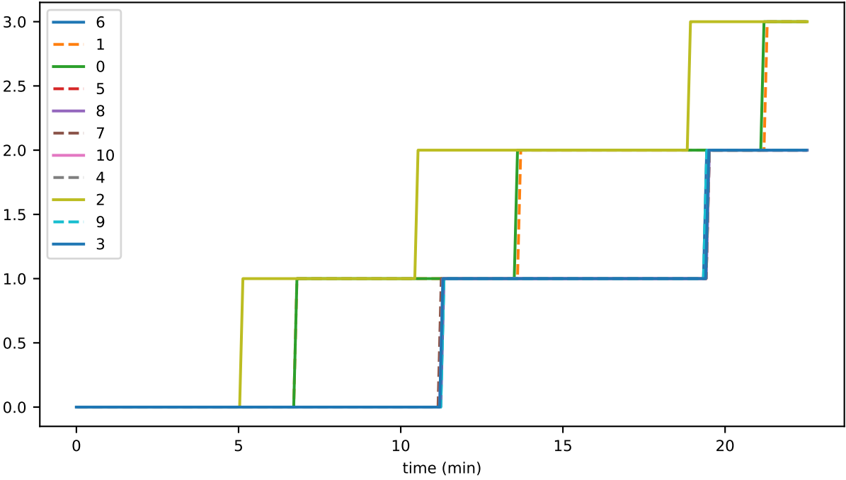
vmap_lifecycle_flushCount_accounts
