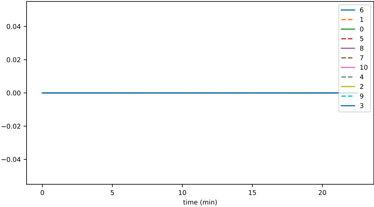
vmap_lifecycle_flushDurationMs_accounts
