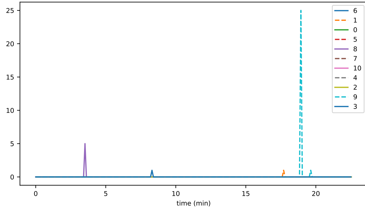
eventRecRate
