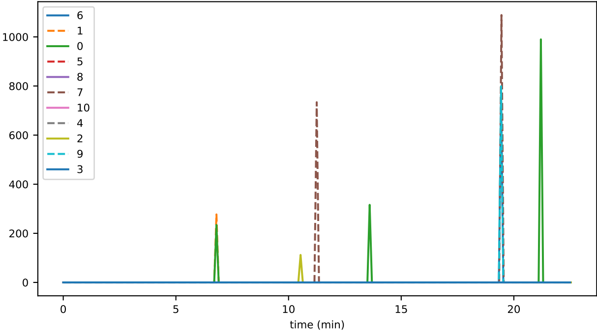
vmap_lifecycle_flushDurationMs_accounts
