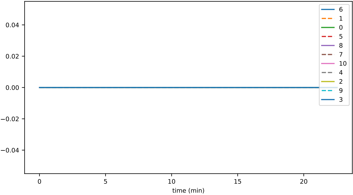
vmap_lifecycle_flushCount_accounts
