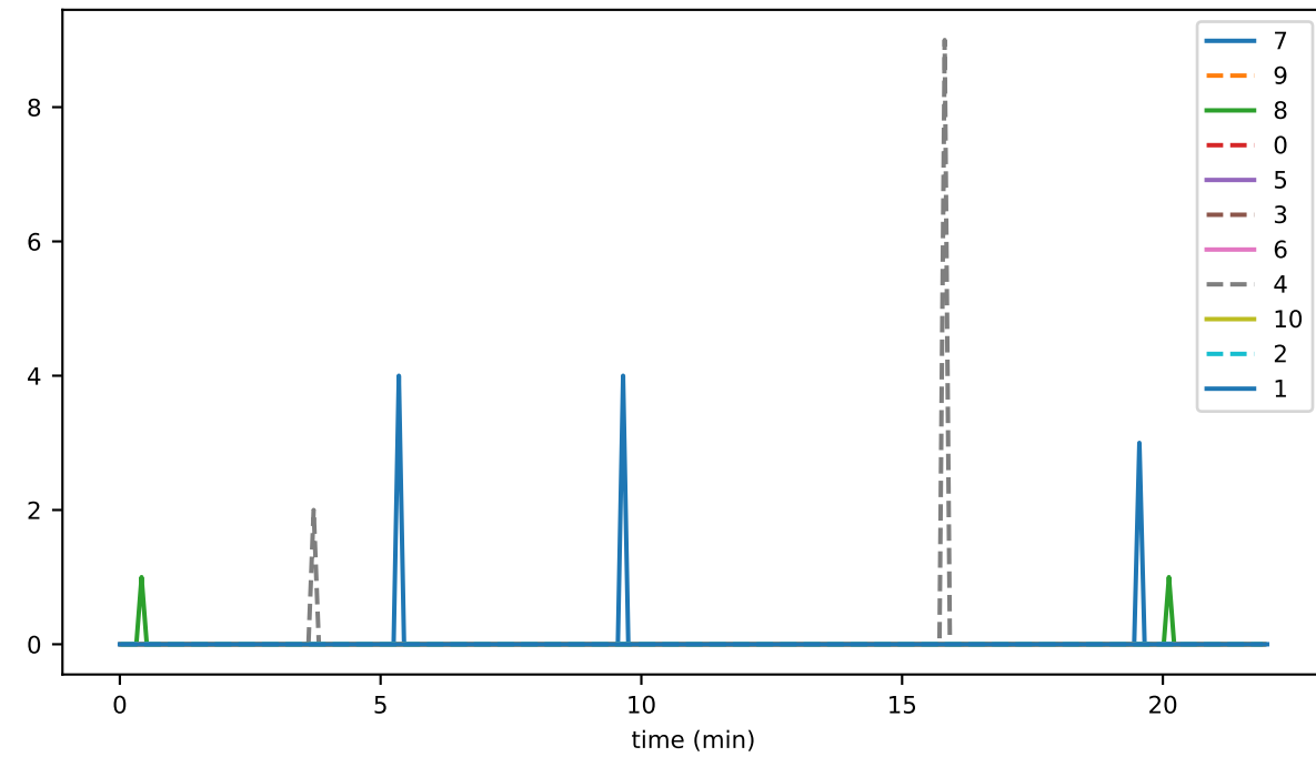
eventRecRate
