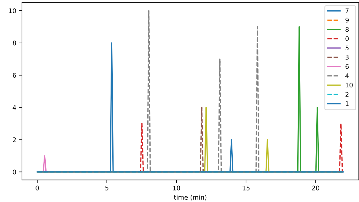
events_per_sec
