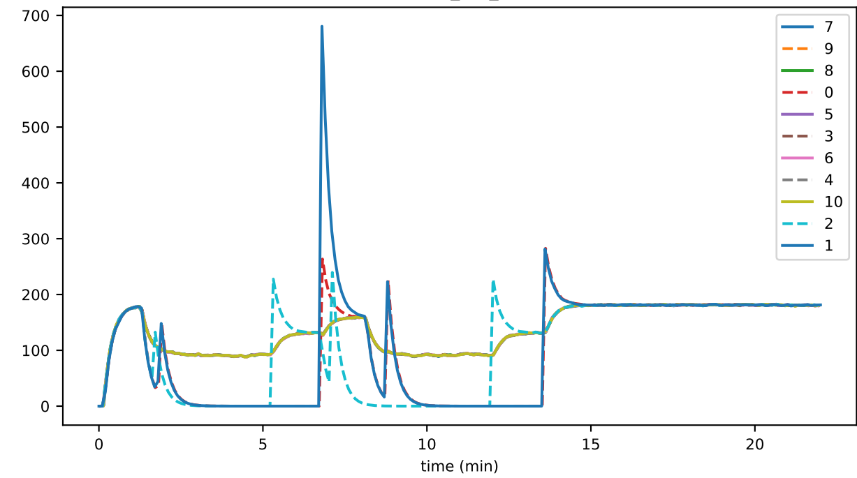
events_per_sec
