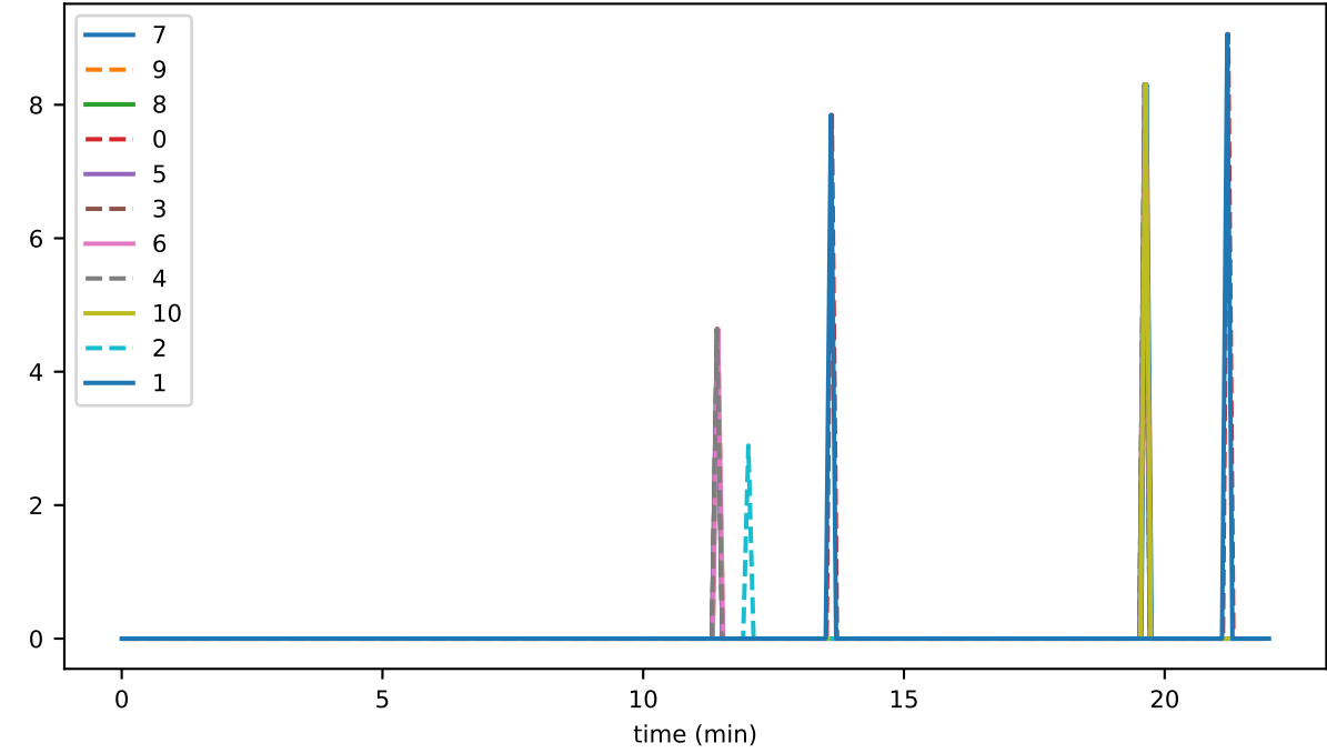
ds_flushes_leafKeysStoreFileSizeMb_accounts
