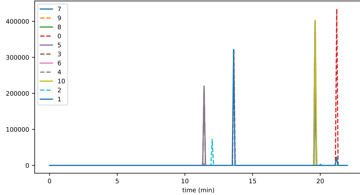
ds_flushes_hashesWritten_accounts
