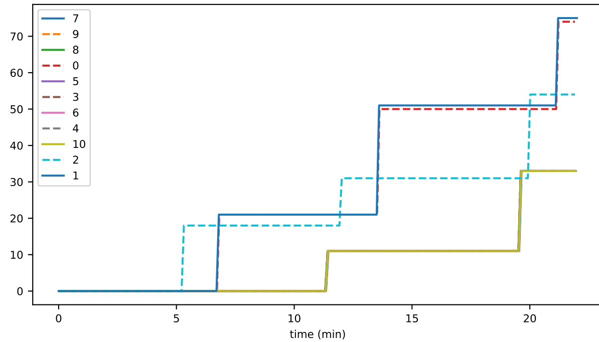
ds_flushes_hashesWritten_accounts
