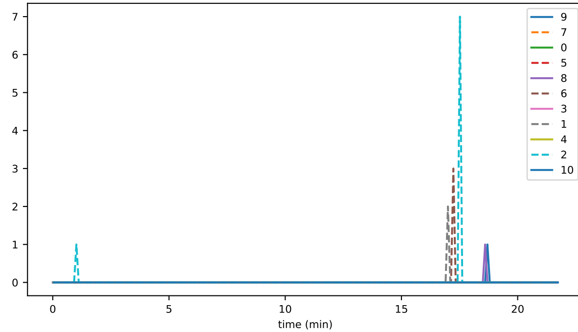
eventRecRate
