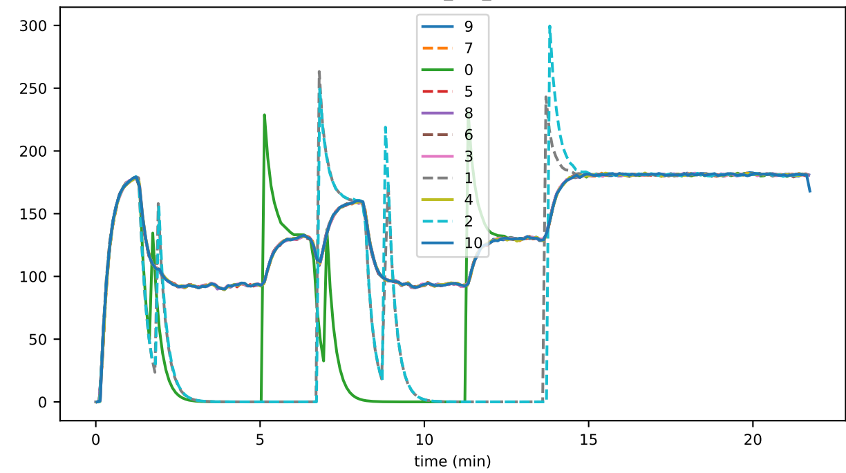
events_per_sec
