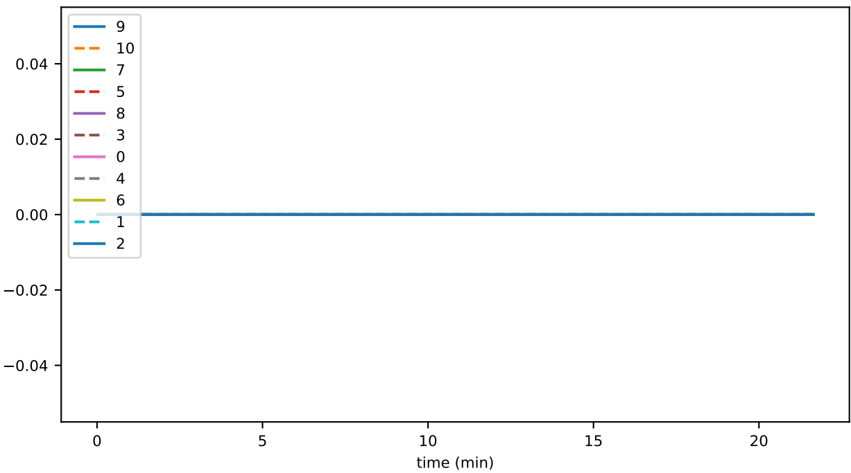
branchingNodeCount
