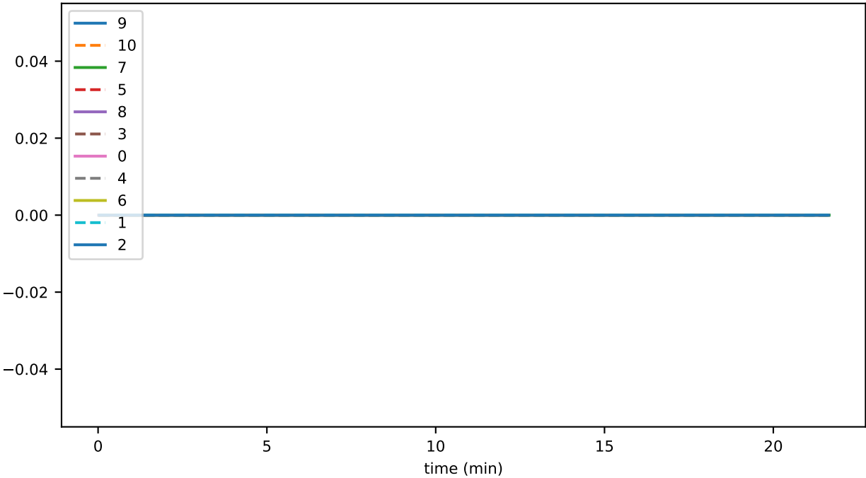
ds_files_level_4_leafKeysFileSizeByLevelMb_accounts
