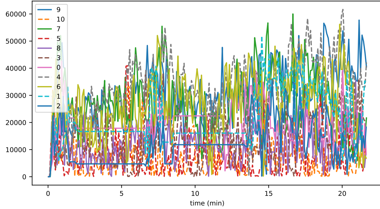
eventRecRate
