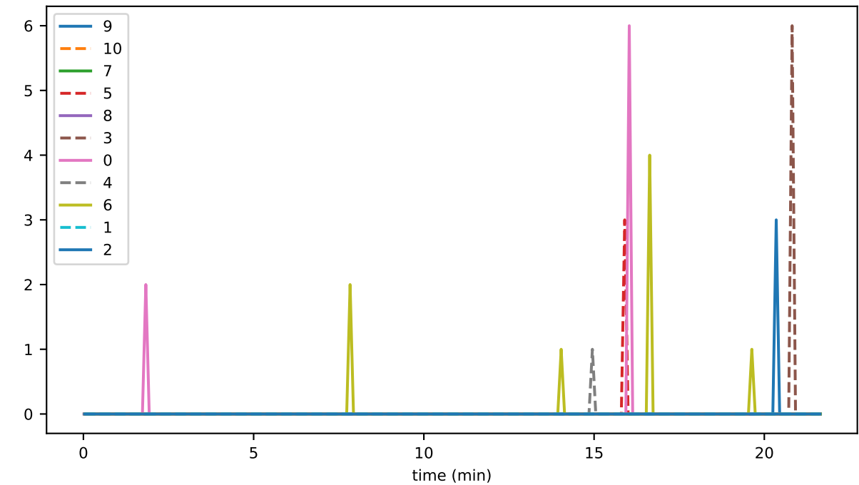
branchingNodeCount
