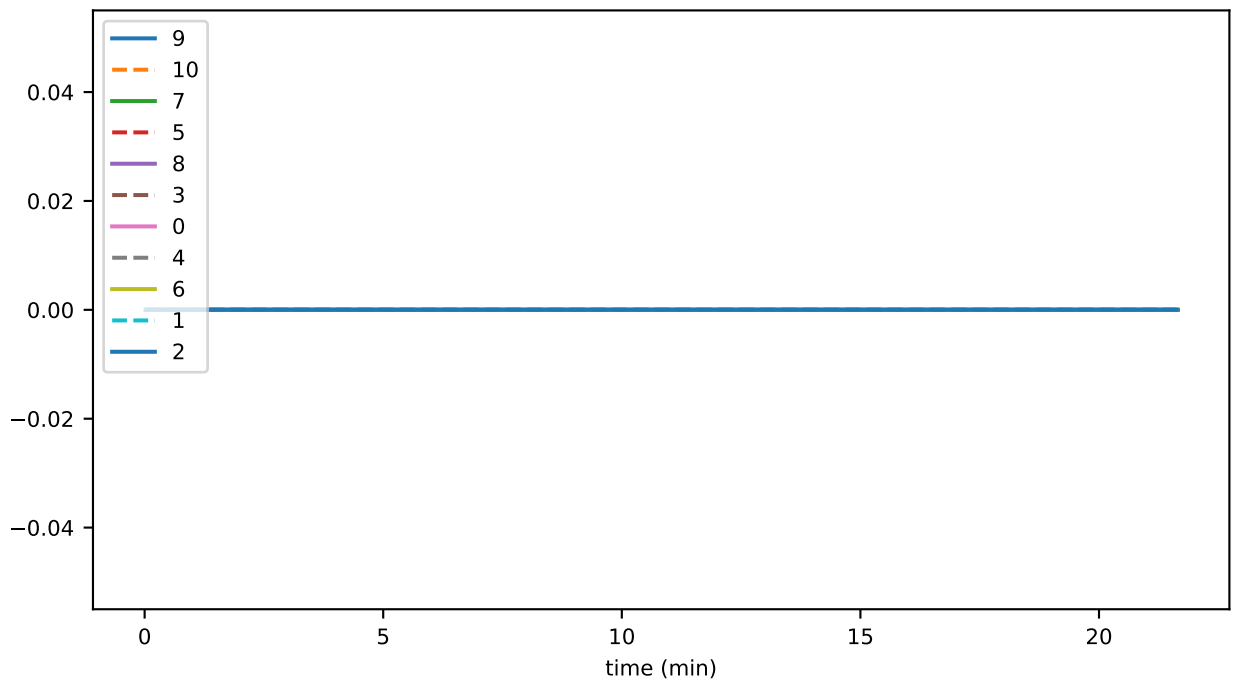
branchingWeightFraction
