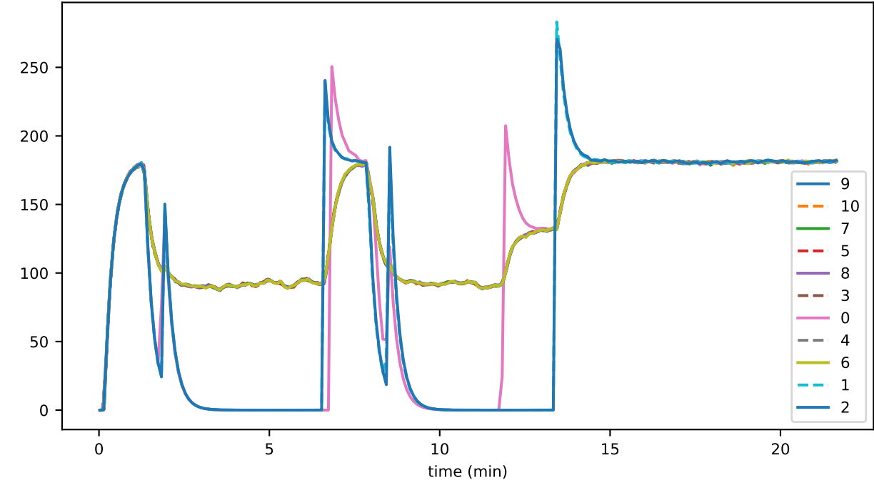
events_per_sec
