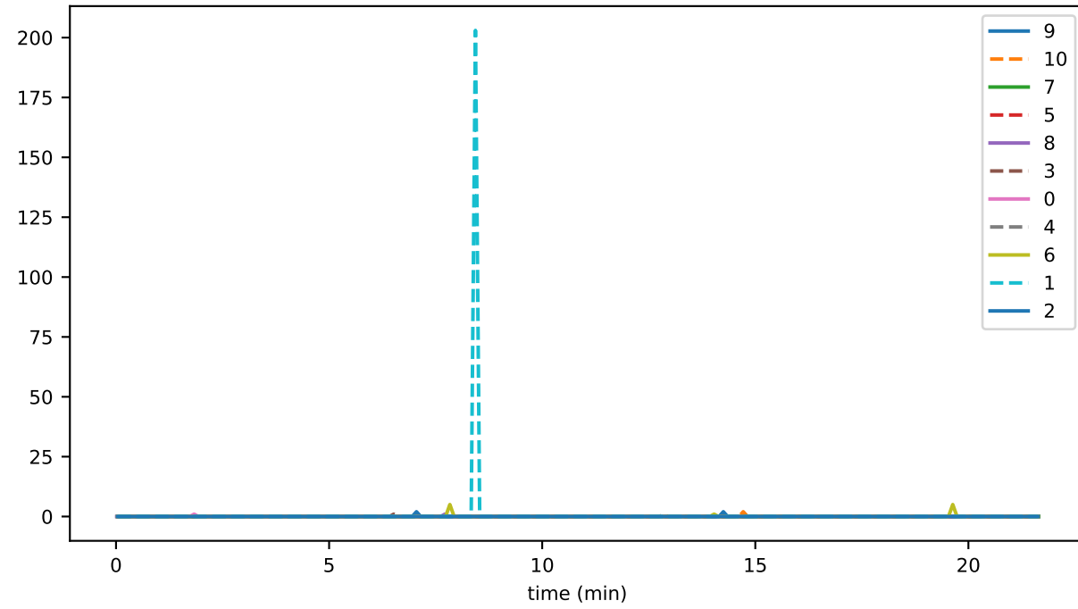
eventRecRate
