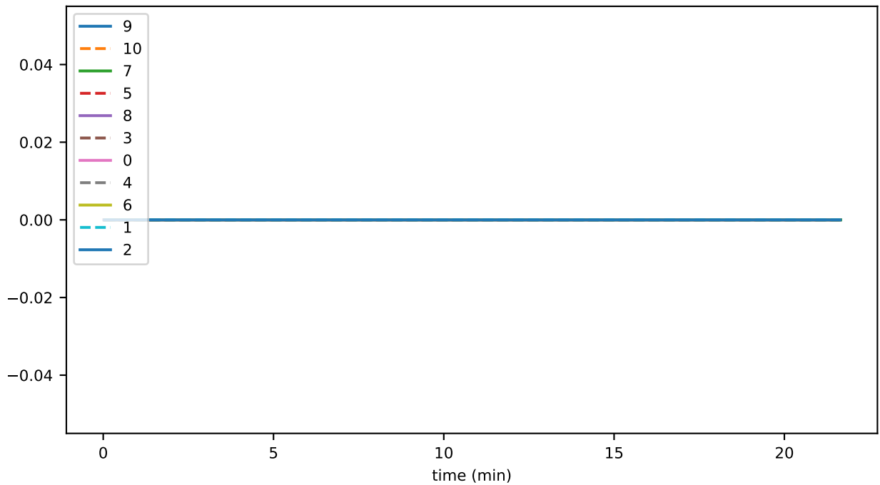
branchingWeightFraction
