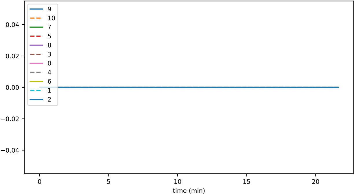
ds_files_level_4_hashesFileSizeByLevelMb_accounts
