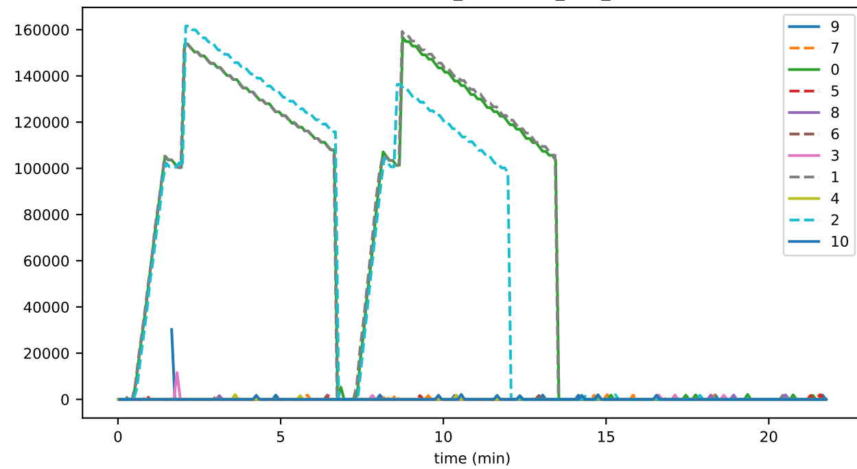
TransactionResubmitter_unhandled_task_count
