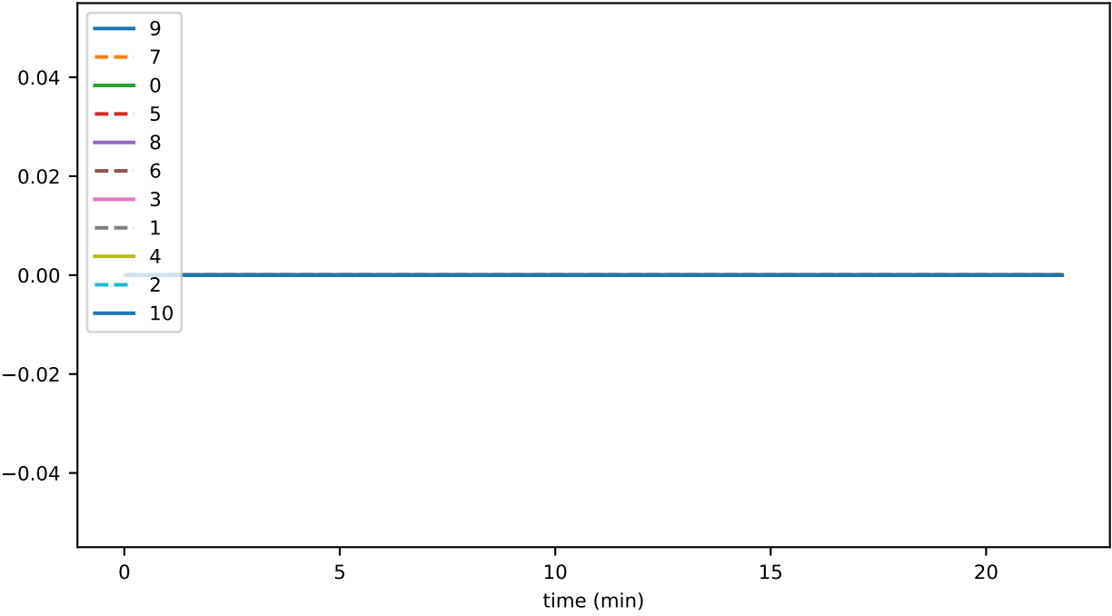
vmap_lifecycle_familySizeBackpressureMs_accounts
