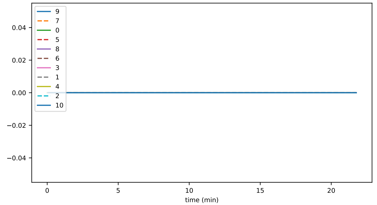
transferredTokensPerSecond
