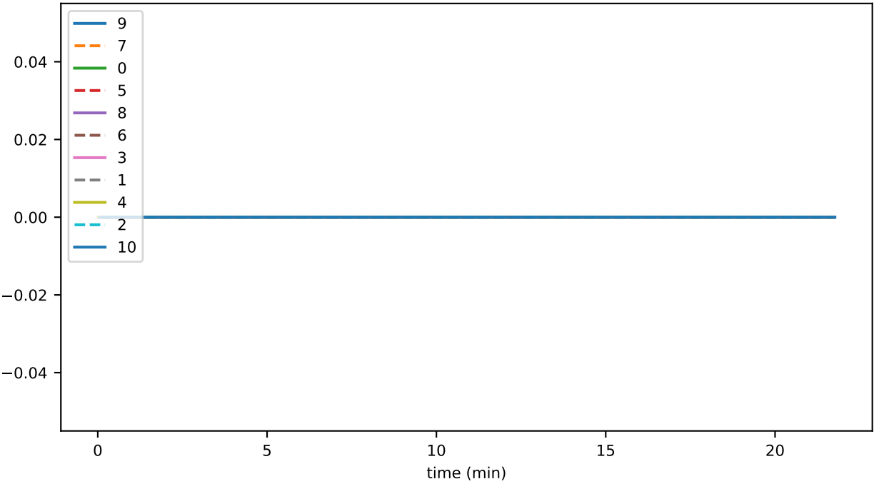
ds_compactions_level_1_leavesTimeMs_accounts
