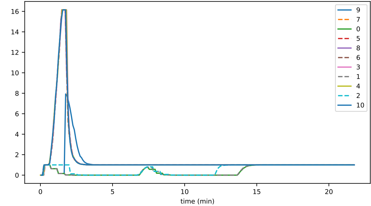
vmap_lifecycle_familySizeBackpressureMs_accounts
