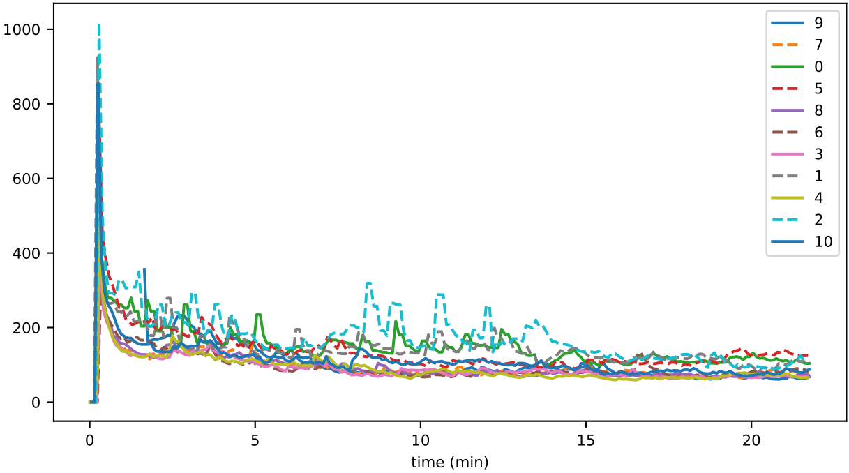
vmap_lifecycle_flushBackpressureMs_accounts
