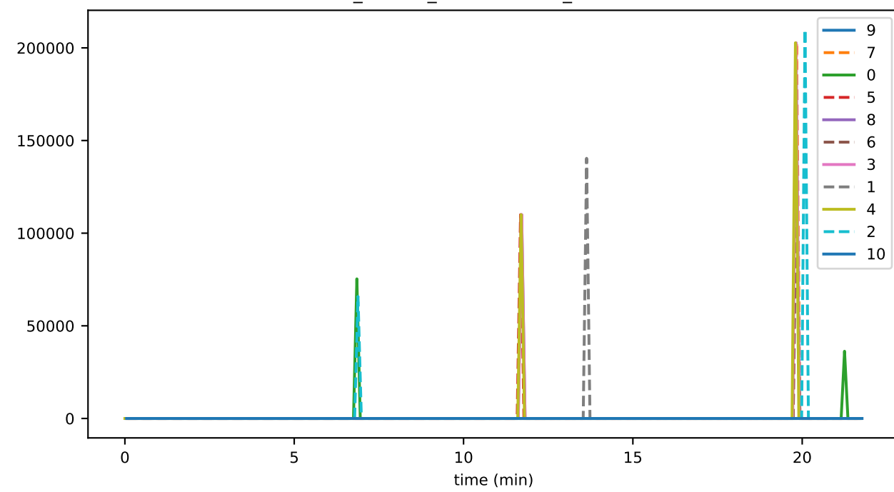
ds_flushes_leavesWritten_accounts
