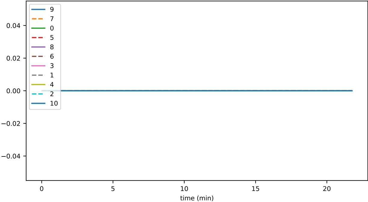
ds_files_level_3_leafKeysFileSizeByLevelMb_accounts
