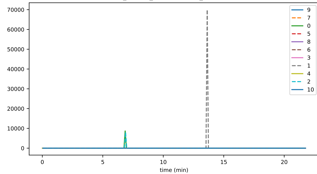
ds_flushes_leavesWritten_accounts
