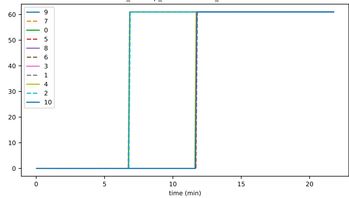
ds_offheap_dataSourceMb_accounts
