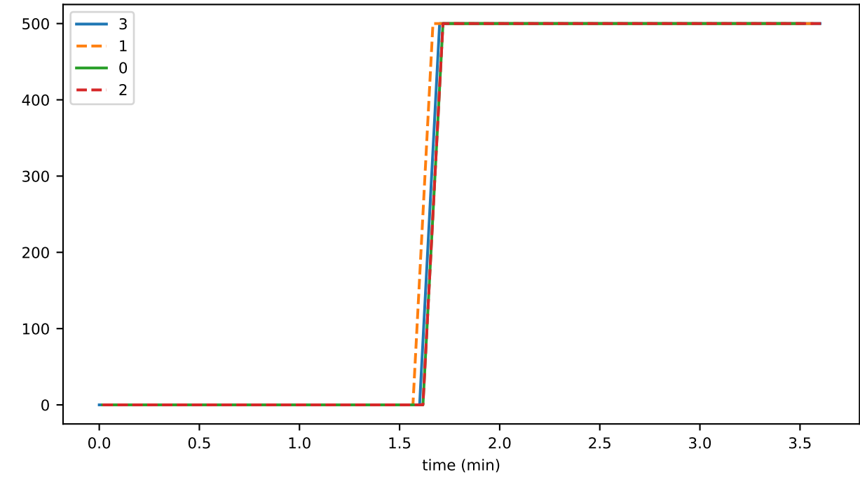
preconsensusEventAverageFileSpan
