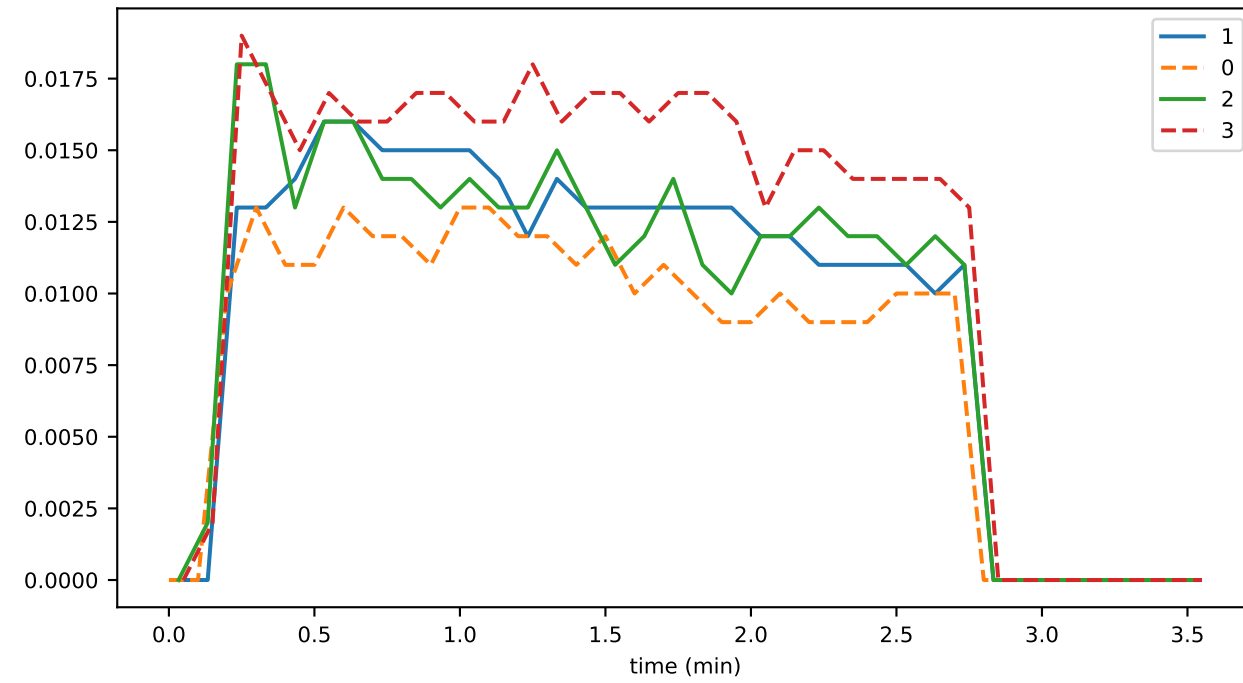
InlinePcesWriter_busy_fraction
