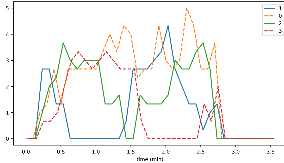
InlinePcesWriter_busy_fraction
