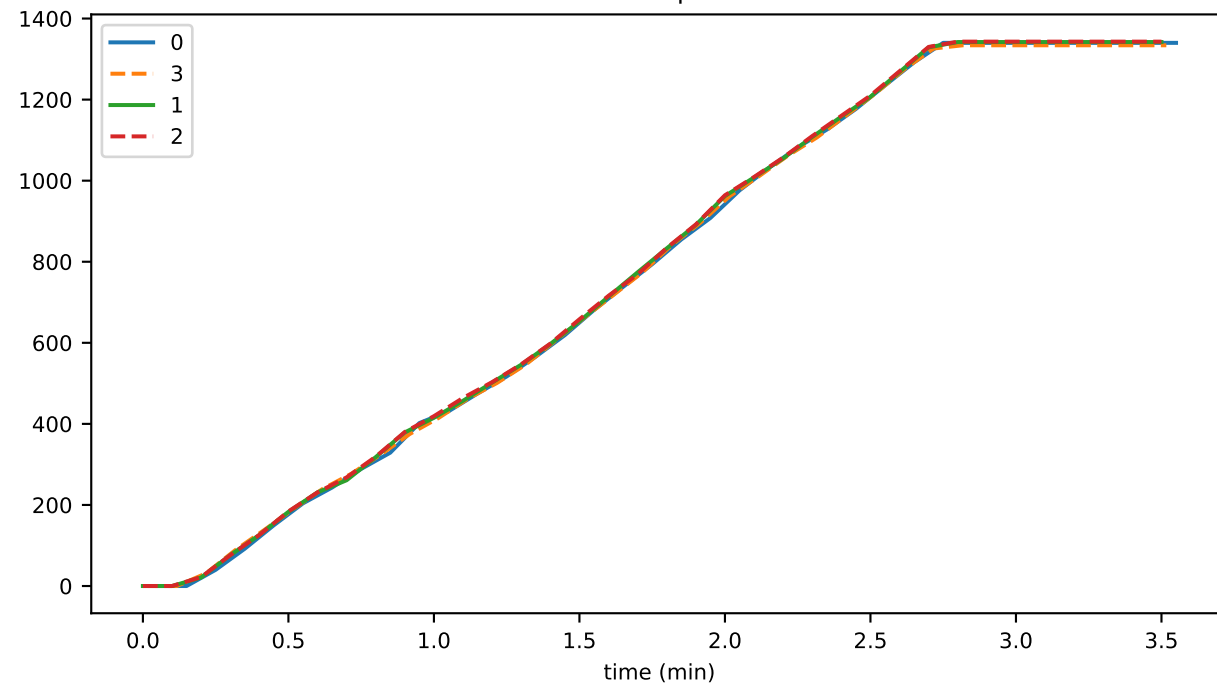
roundIncEqParents
