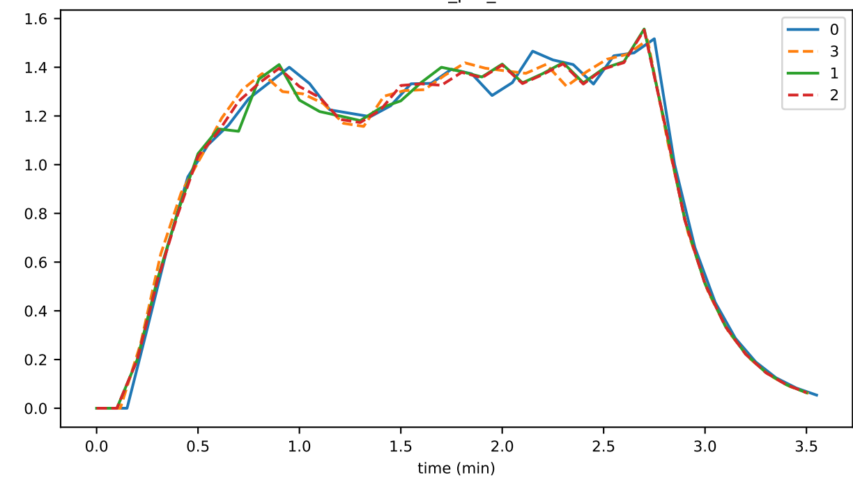
rounds_per_sec
