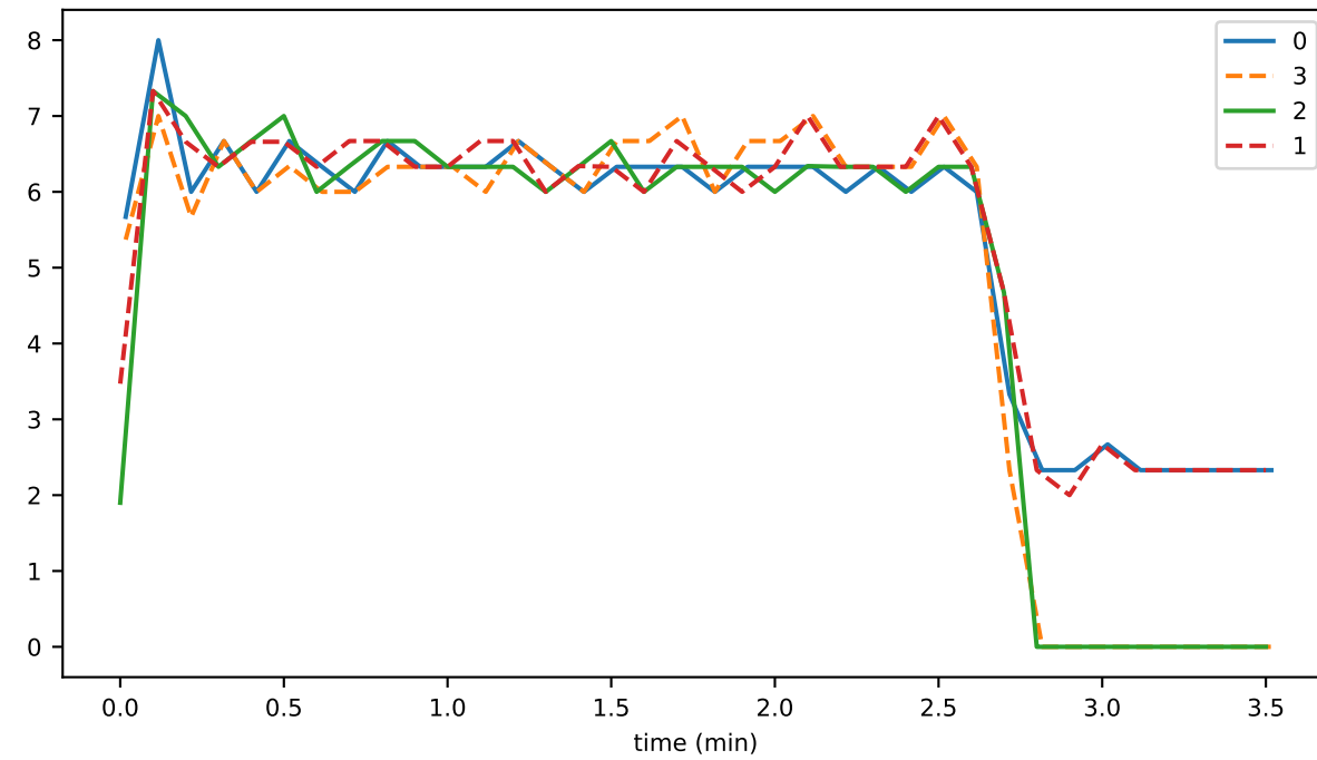
orphanBufferSize
