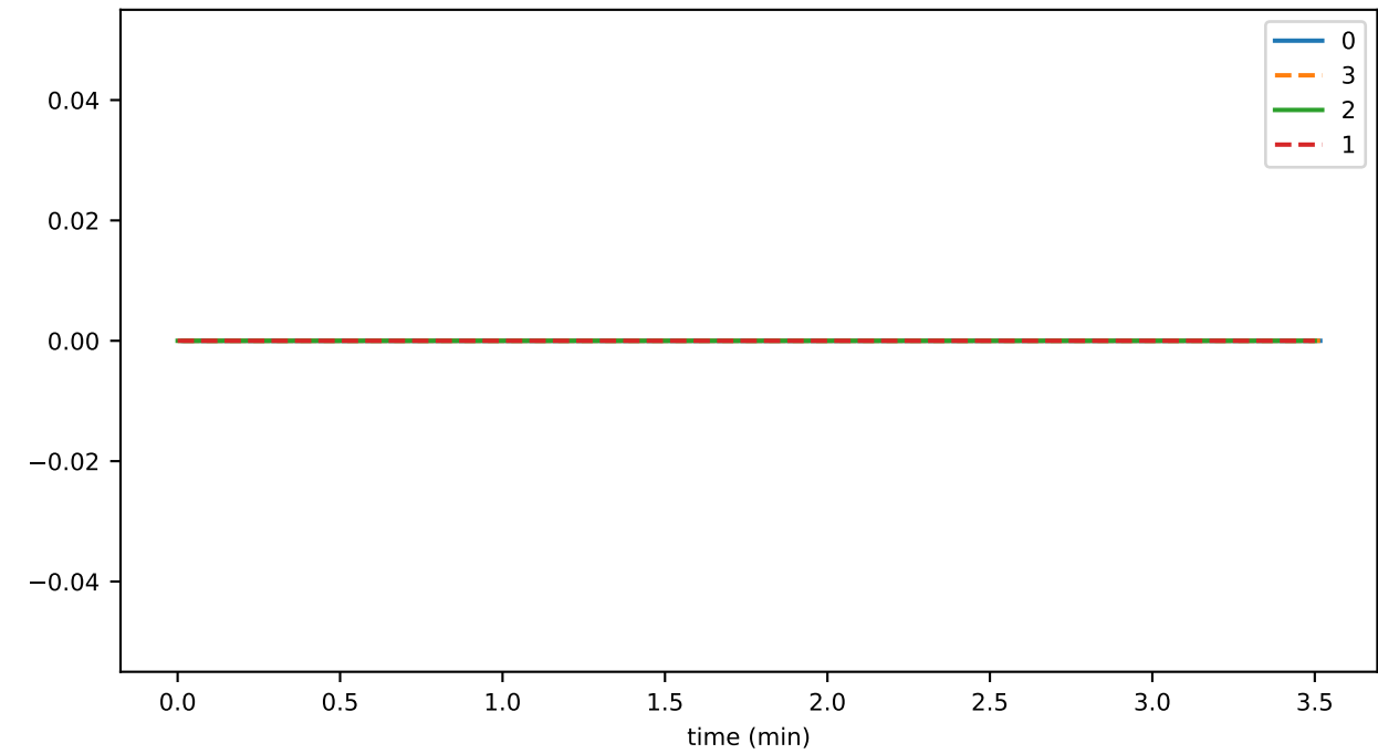
outgoingSyncRequests_per_sec
