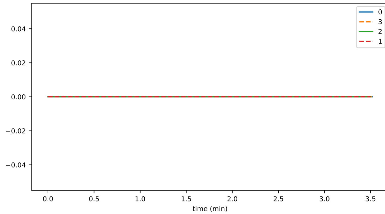
orphanBufferSize
