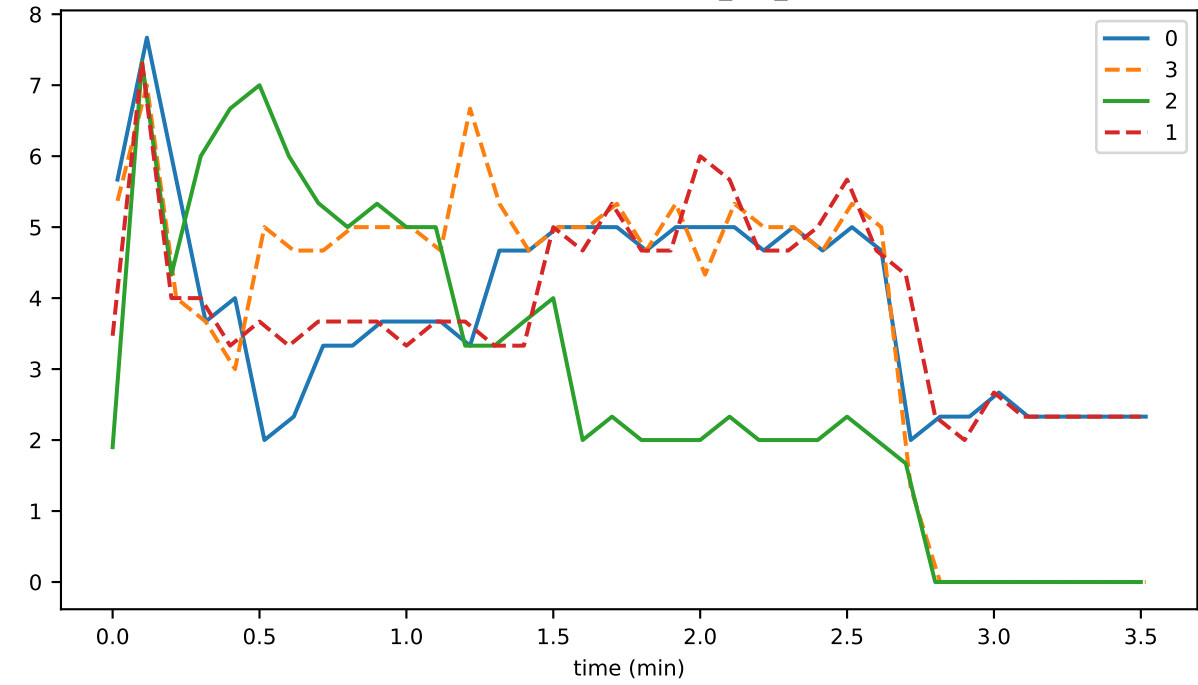
outgoingSyncRequests_per_sec
