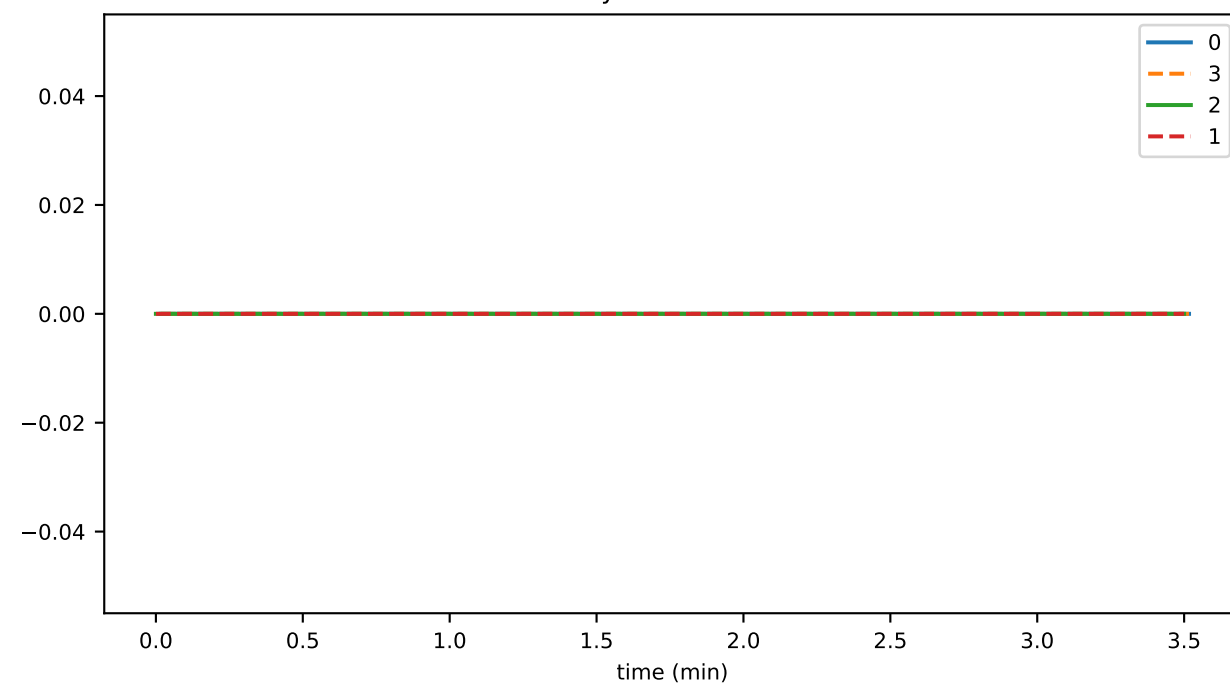
doNotSyncPlatformStatus
