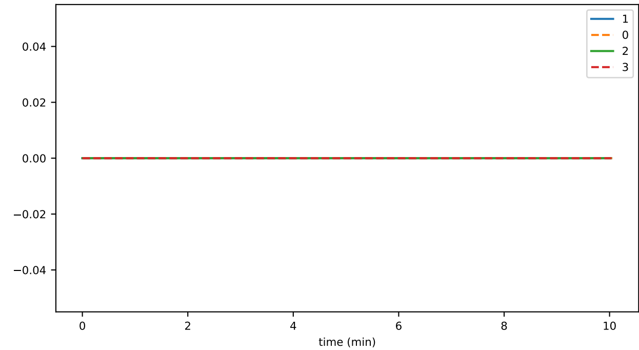
rounds_per_sec
