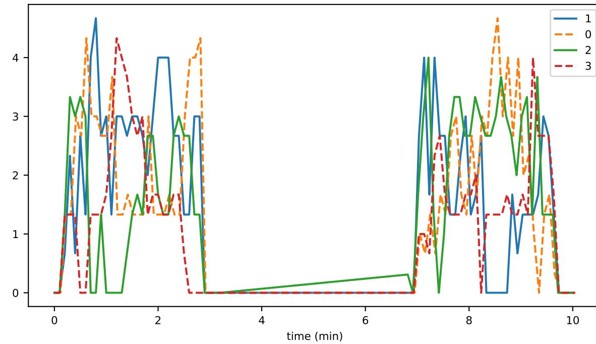
doNotSyncPlatformStatus
