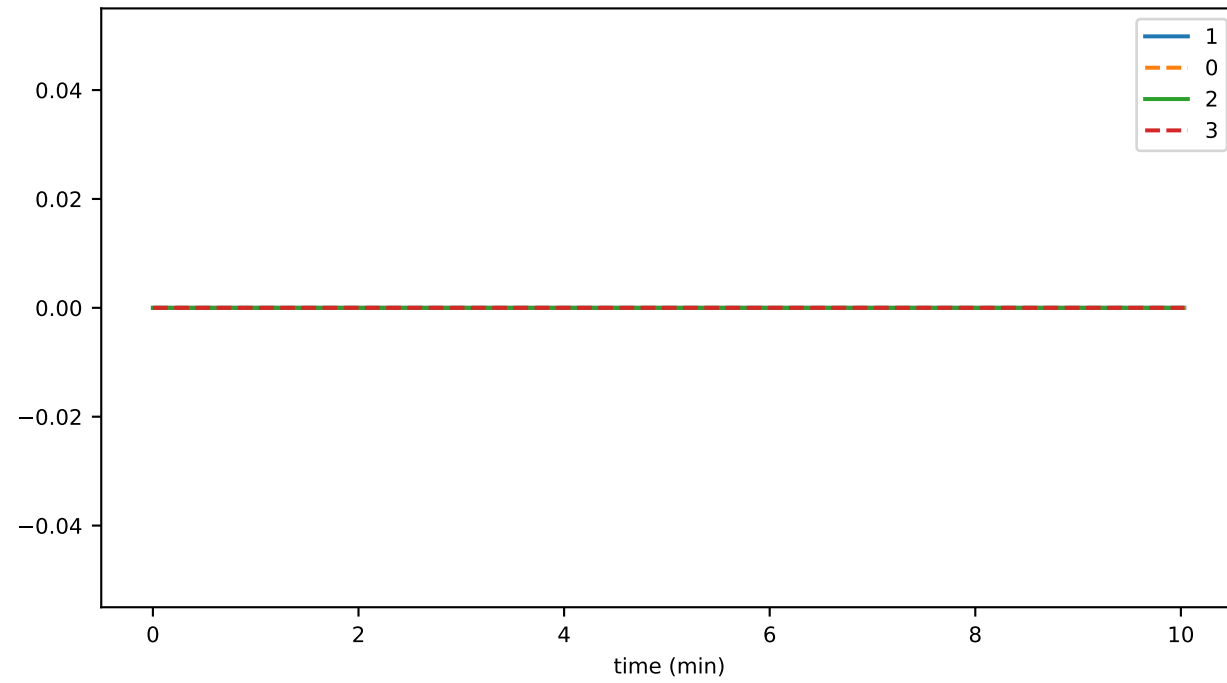
doNotSyncPlatformStatus
