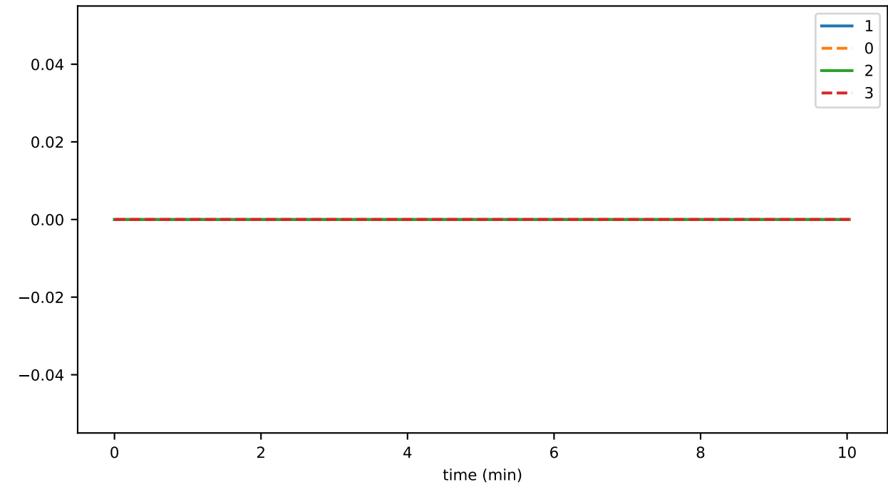
doNotSyncRemoteFallenBehind
