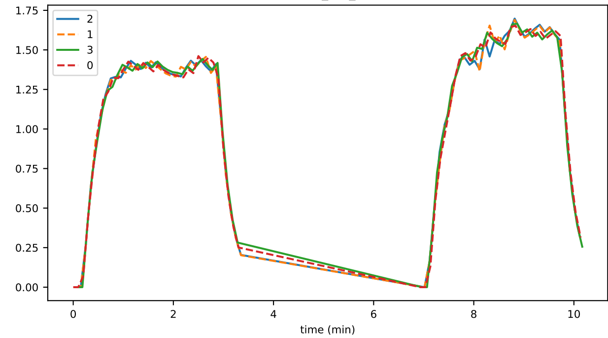
rounds_per_sec
