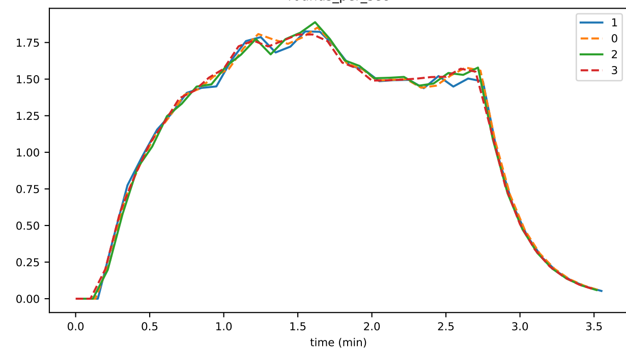
rounds_per_sec
