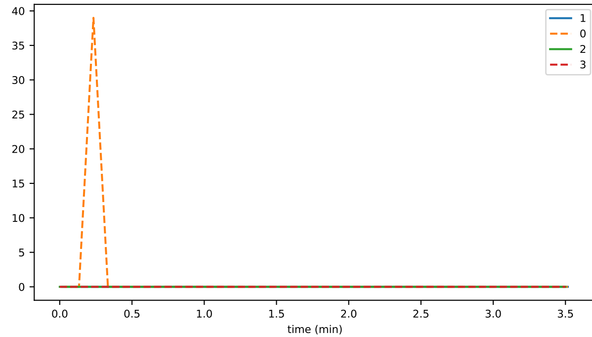
TransactionResubmitter_unhandled_task_count
