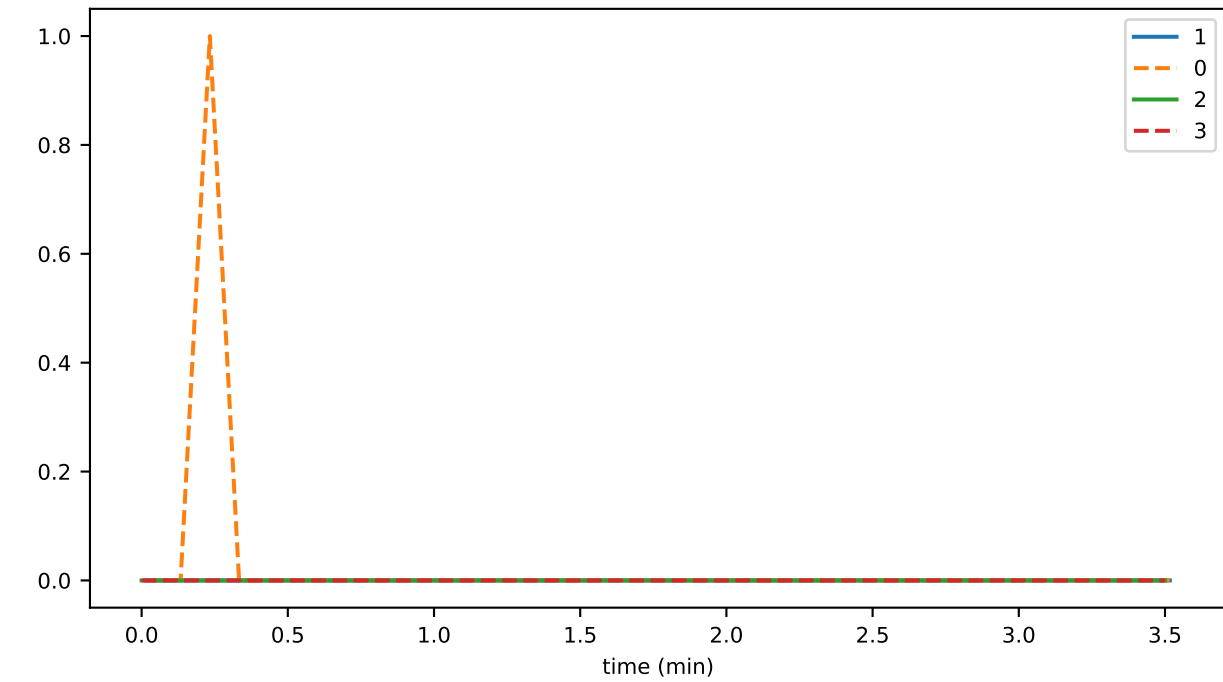
transferredTokensPerSecond
