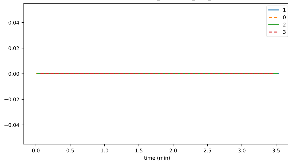
TransactionResubmitter_unhandled_task_count
