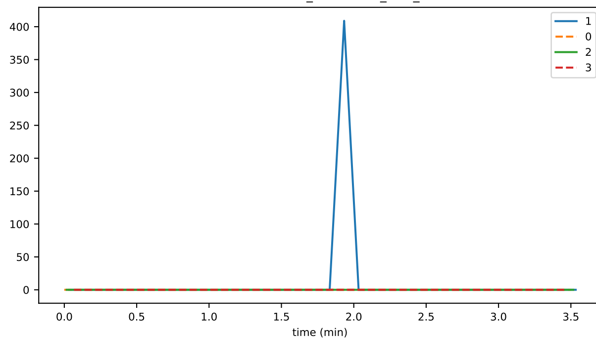
TransactionResubmitter_unhandled_task_count
