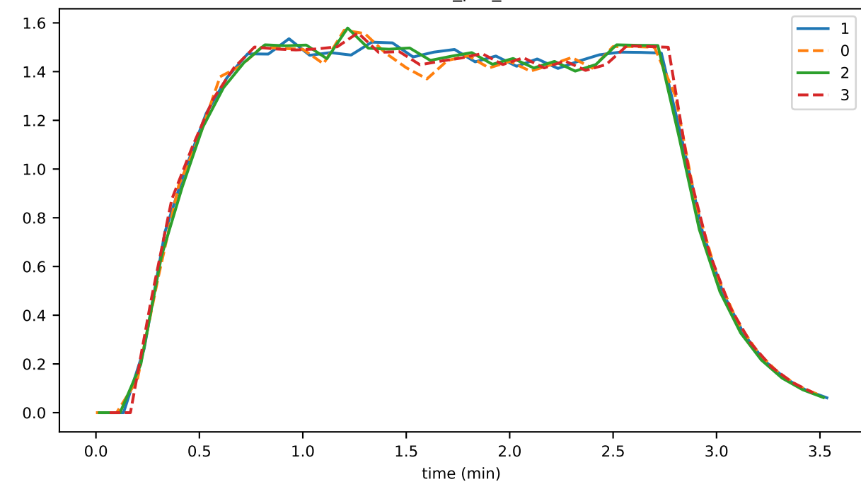
rounds_per_sec
