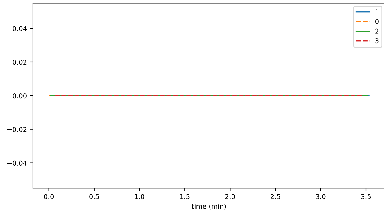
doNotSyncRemoteFallenBehind
