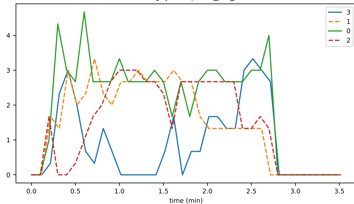
InlinePcesWriter_busy_fraction
