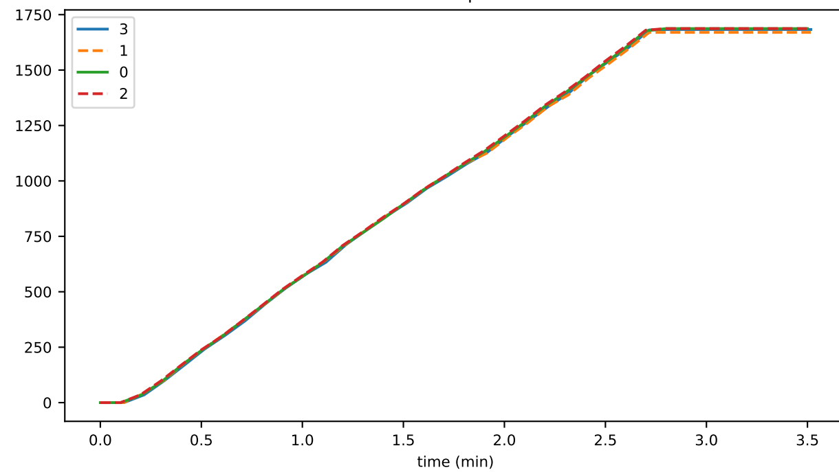
roundIncEqParents
