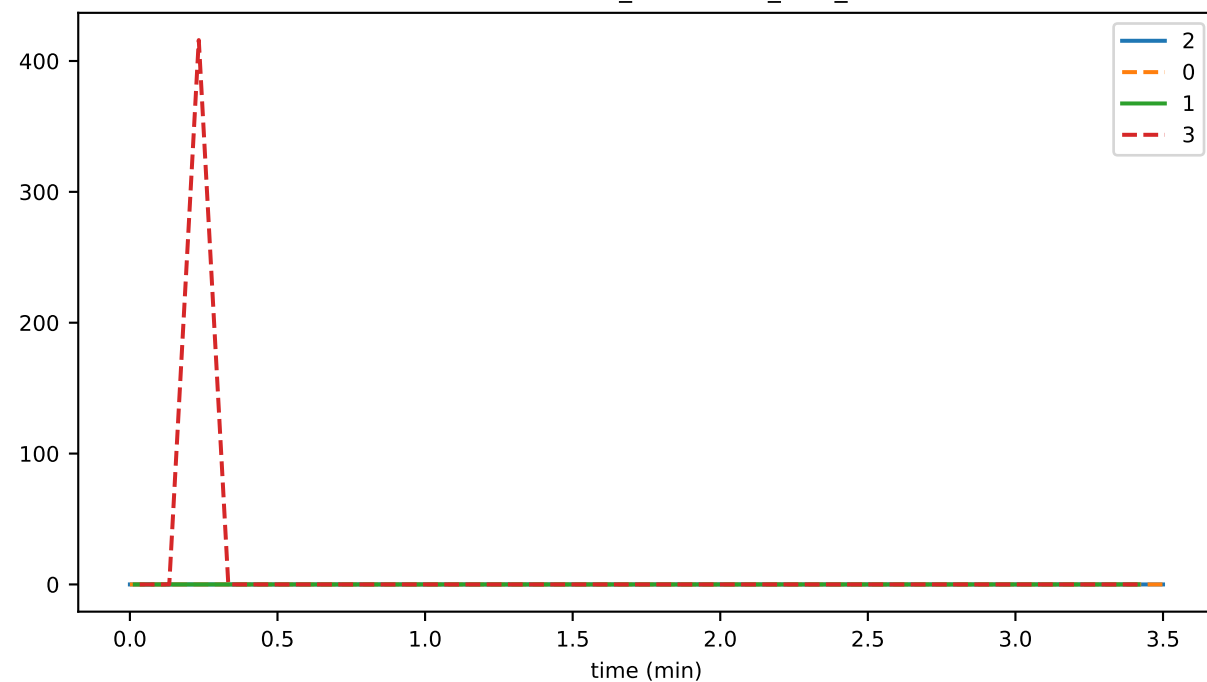
TransactionResubmitter_unhandled_task_count
