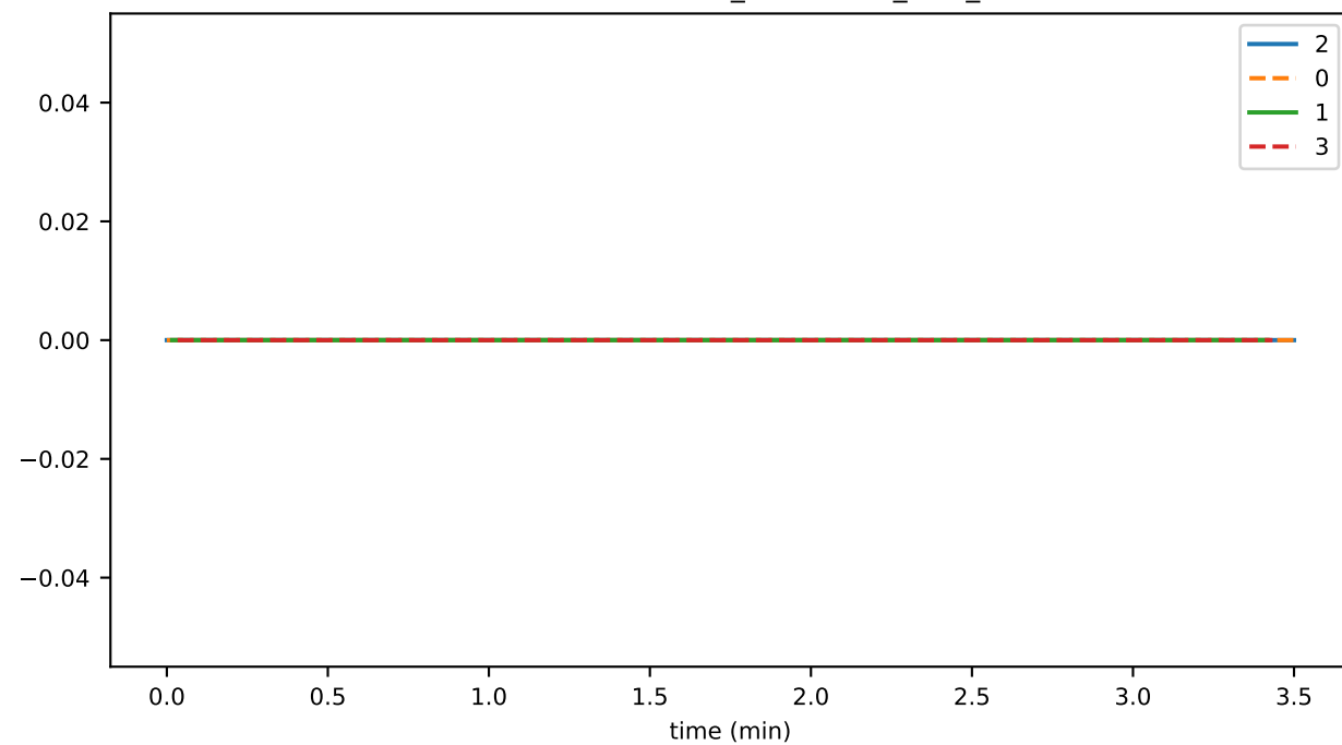
TransactionResubmitter_unhandled_task_count
