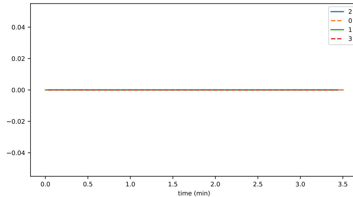
transferredTokensPerSecond
