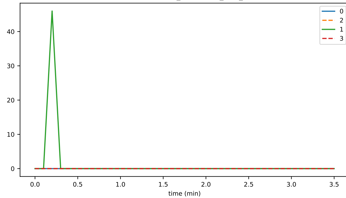
TransactionResubmitter_unhandled_task_count
