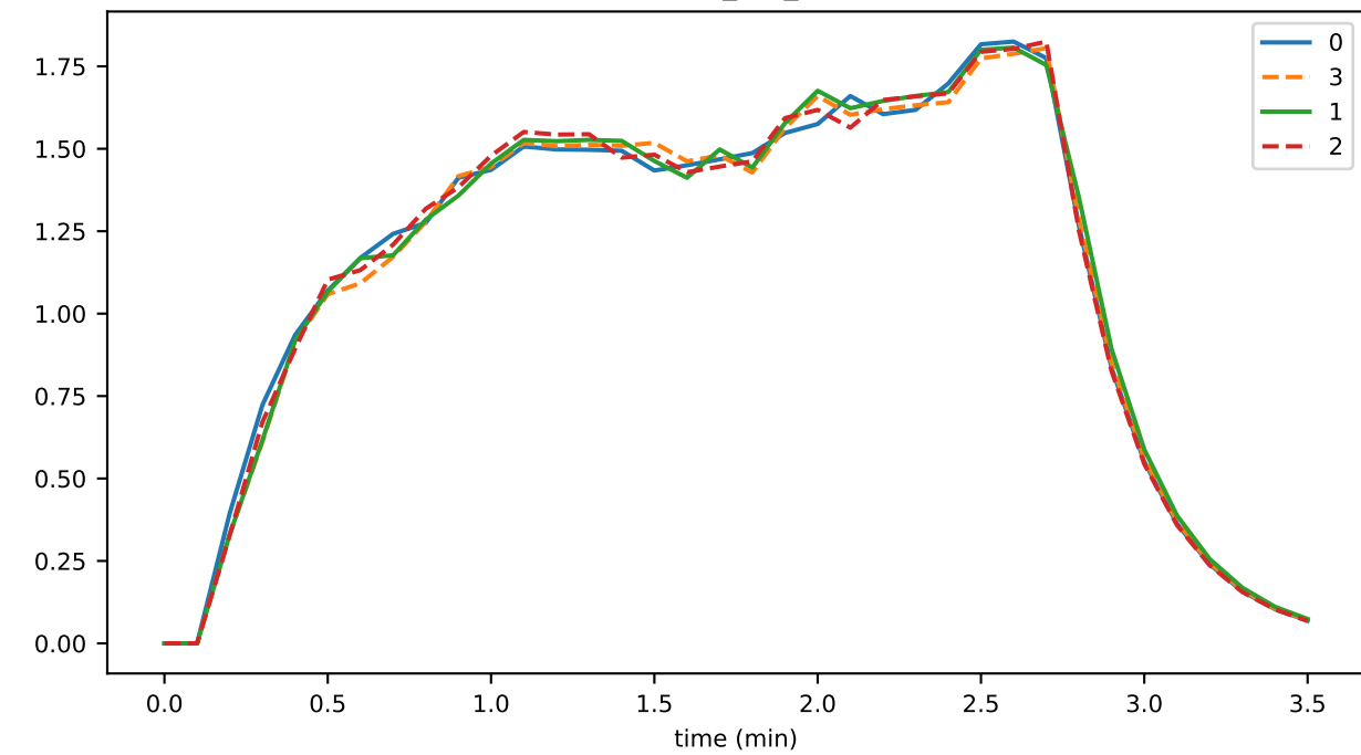
rounds_per_sec
